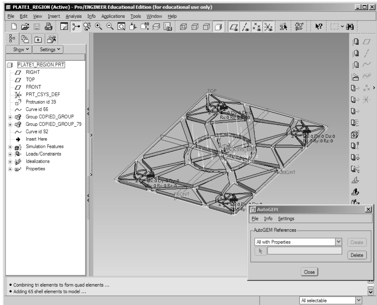
PRO/MECHANICA Mesh of a Sheet Metal Plate
