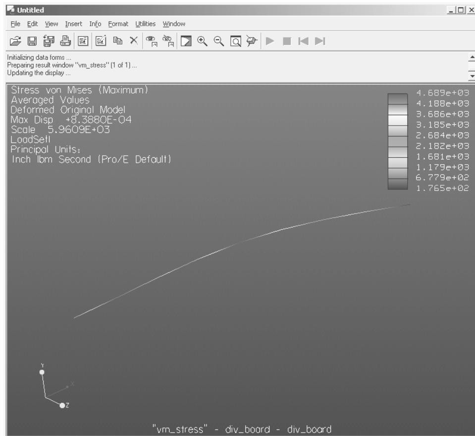
Figure 40: Von Mises Stress fringe plot for Project 1
