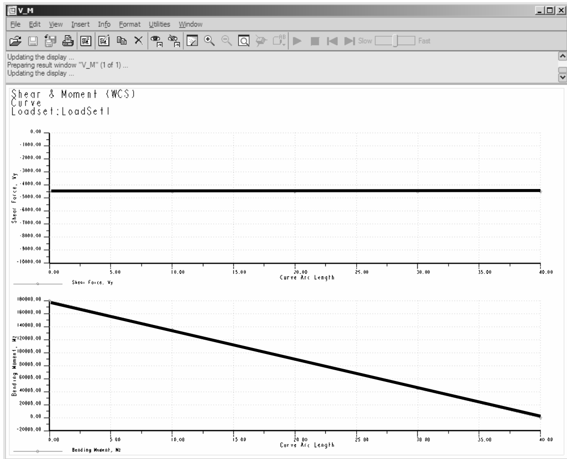
Figure 37: Shear and moment diagrams
