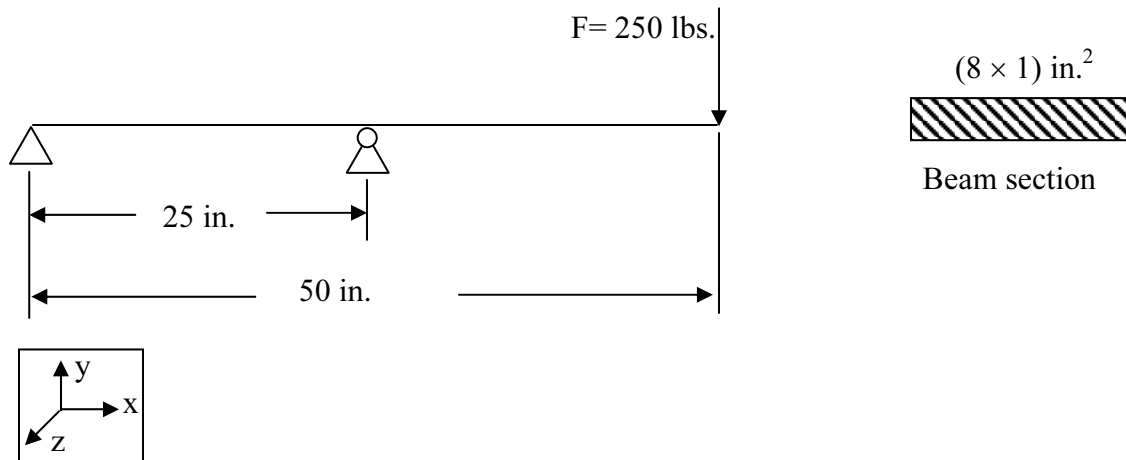
Figure 38: Diving Board Loading Diagram
