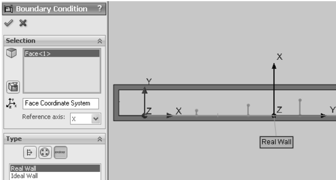
Figure 2.20 Real wall boundary condition for the flat plate
