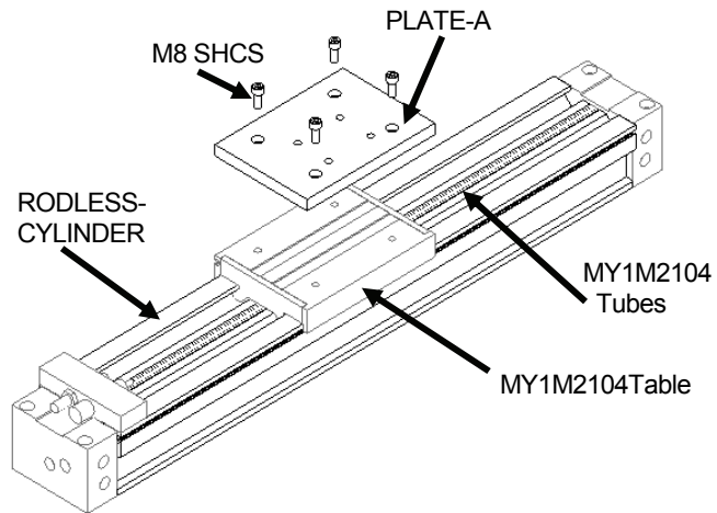
LINEAR-TRANSFER assembly
