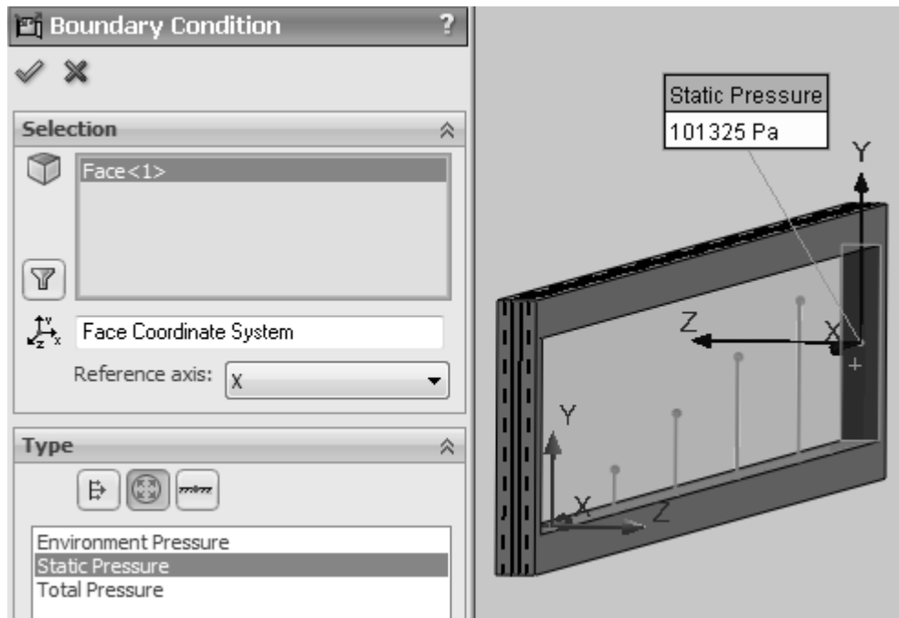
Figure 2.18a) Selection of static pressure as boundary condition at the outlet of the flow region
