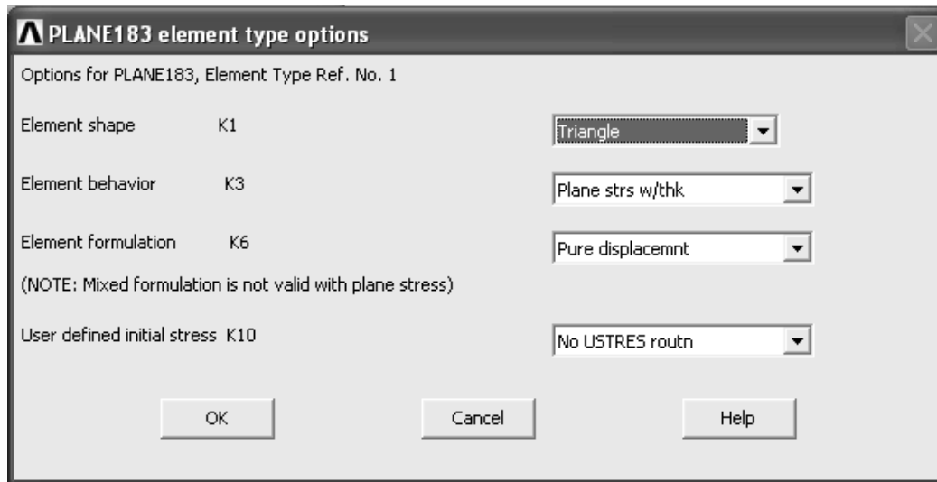
Figure 2-6 Element options.
