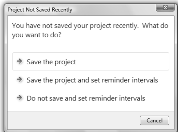
FIGURE 3-2.6 Save reminder
