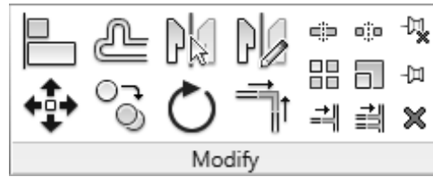
FIGURE 3-3.1 Modify panel
