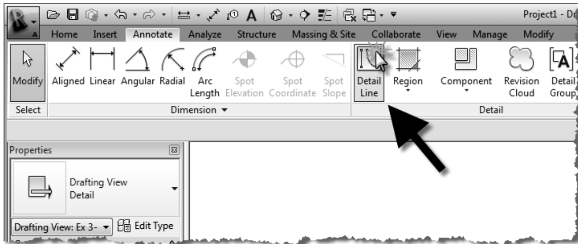
FIGURE 3-1.5 Annotate tab
