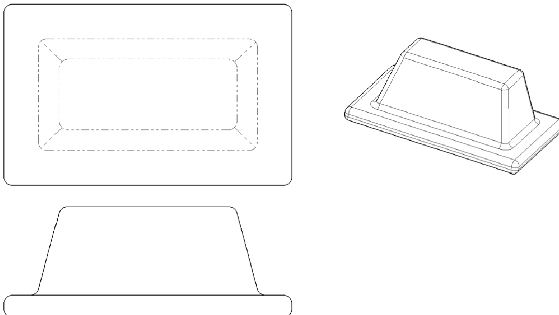
Figure 2.6-10: Phantom lines used to indicated a change in surface direction
