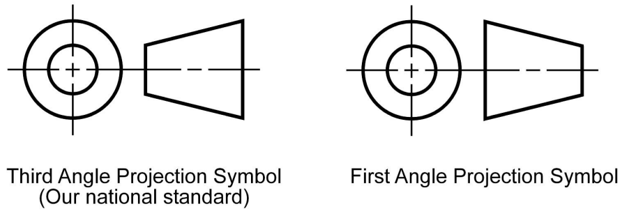
Figure 2.7-2: First and third angle projection symbols.
