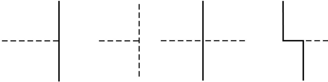
Figure 2.6-1: Drawing hidden lines.
