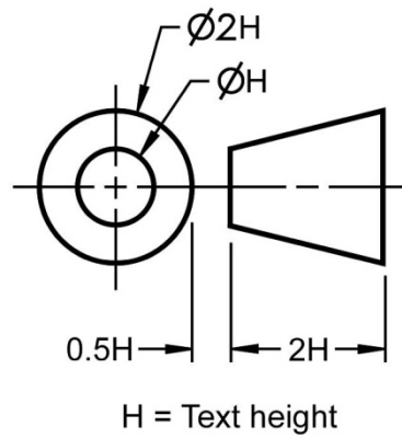
Figure 2.7-3: Projection symbol proportions.
