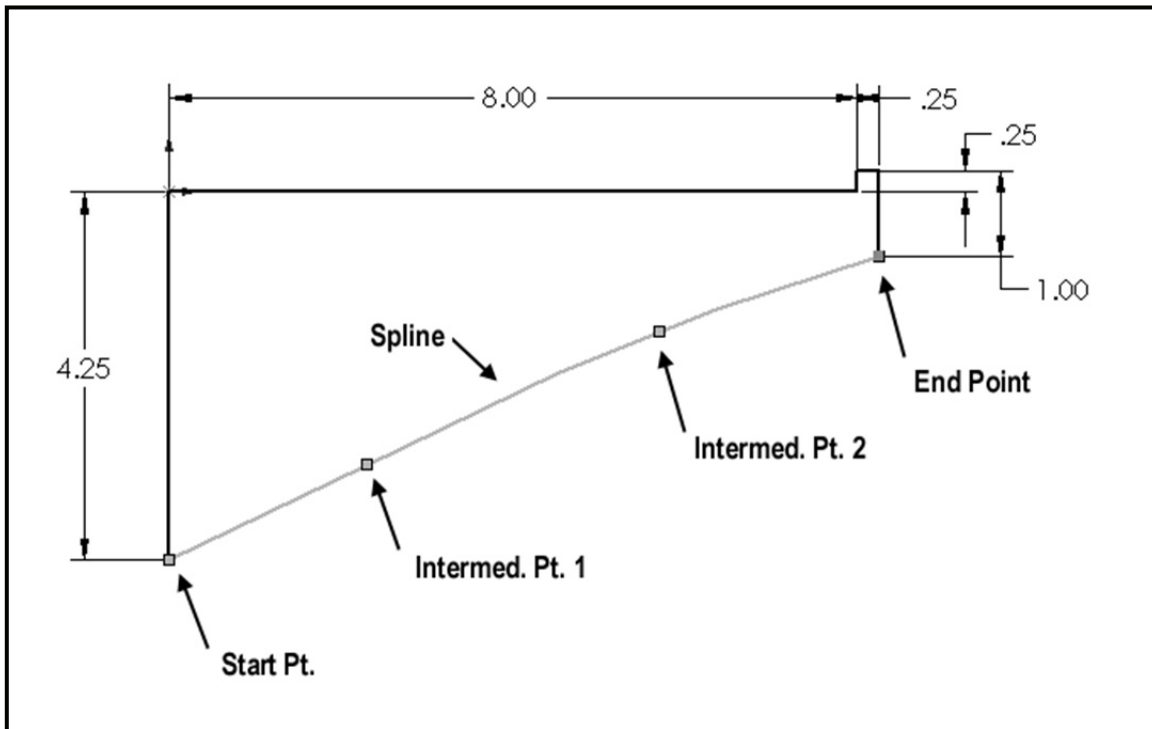
Figure 1-33. Sketching the Spline through its Four Points.
