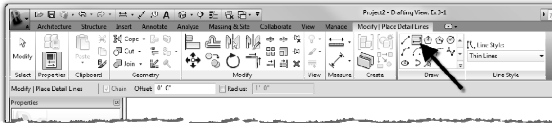
FIGURE 3-1.14 Place Detail Lines contextual Tab on Ribbon
