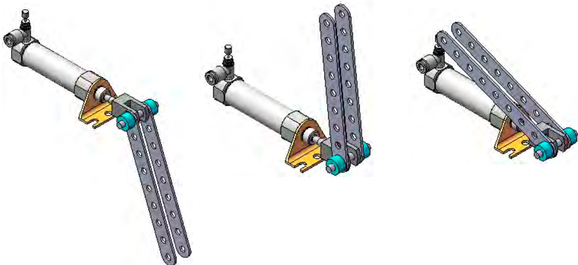
LINKAGE Assembly Basic Simulation
