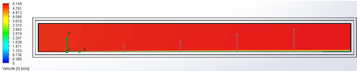
Figure 2.23b) X – Component of Velocity distribution on the flat plate.
