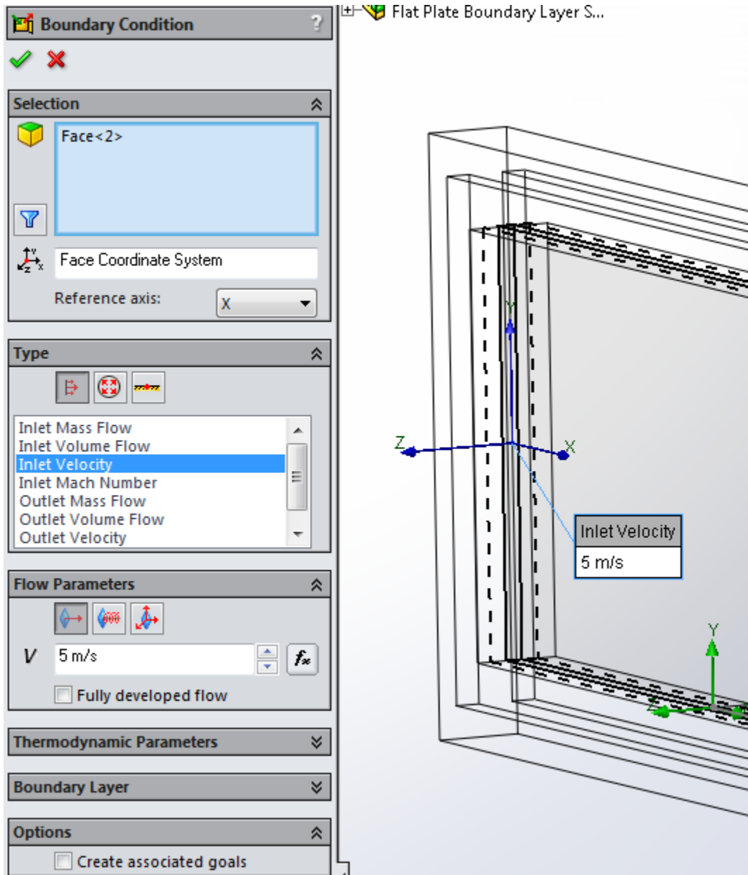
Figure 2.17c) Velocity boundary condition on the inflow
