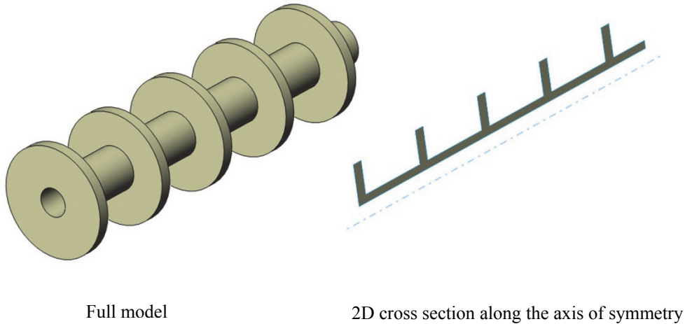
Figure 1-11: Axisymmetric model AXISYM may be represented by a 2D cross section.
