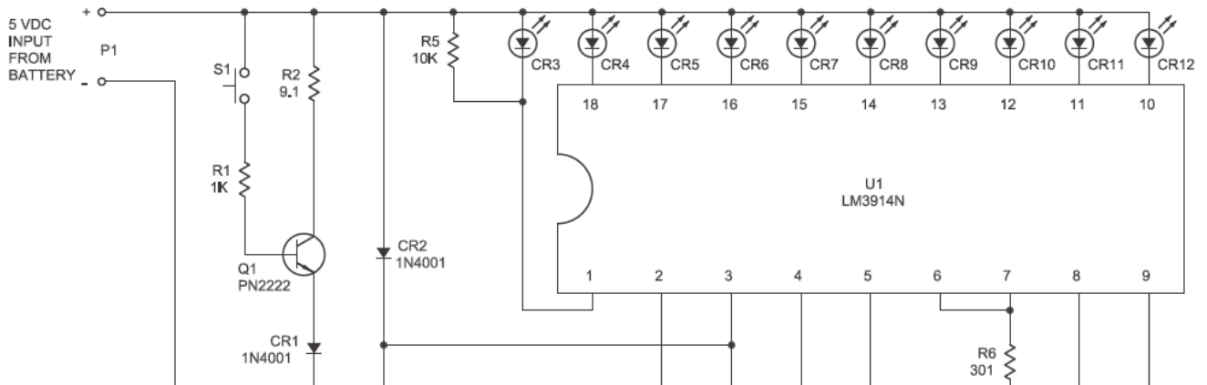
1.7 Detail from an Electronics Schematic
