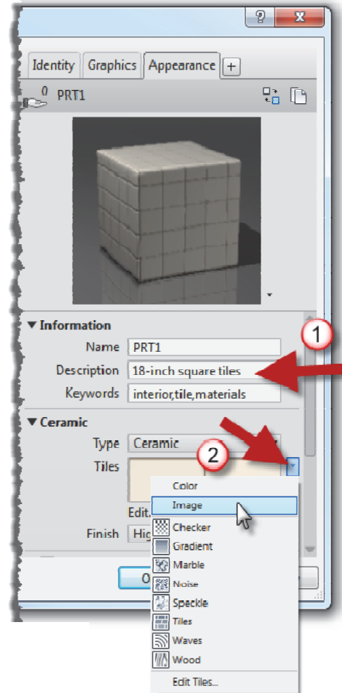
FIGURE 4-4.17 Appearance tab
