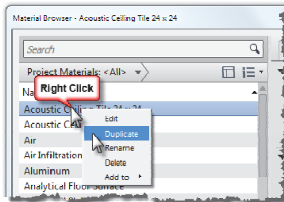
FIGURE 4-2.5 Right-click options
