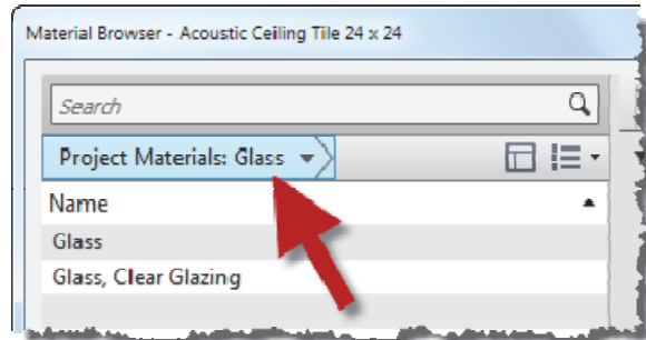
FIGURE 4-2.4B Right-click options
