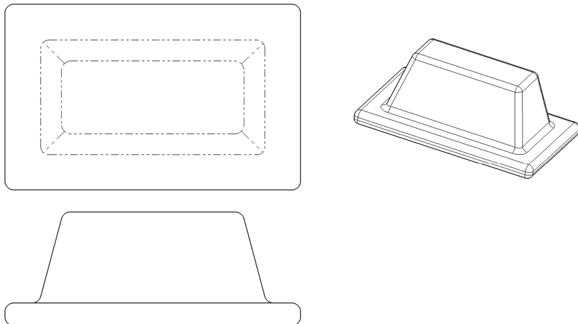
Figure 2.6-10: Phantom lines used to indicate a change in surface direction
