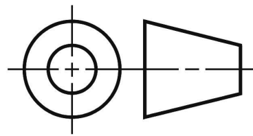
First Angle Projection Symbol
