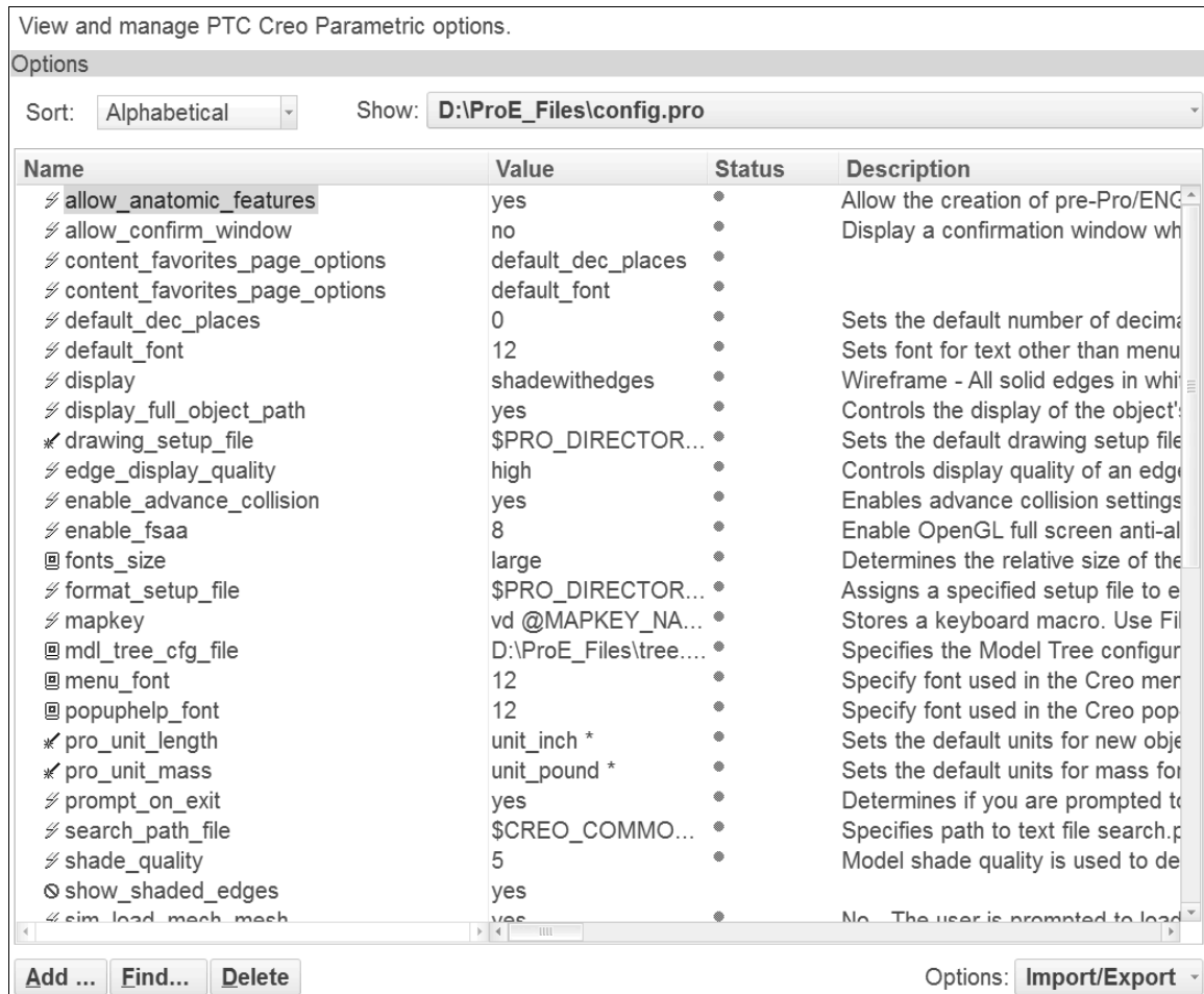
Figure 4 The config.pro file layout showing current settings
