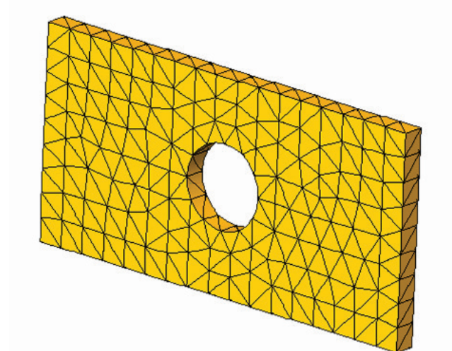
Figure 2-17: A coarse mesh created with second order, solid tetrahedral elements.
