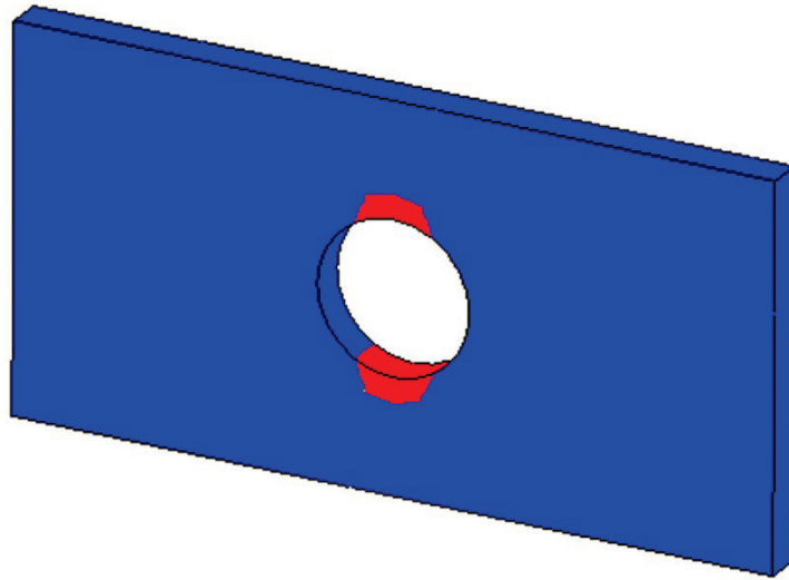
Figure 2-29: The red color displays the areas where the factor of safety falls below 3.
