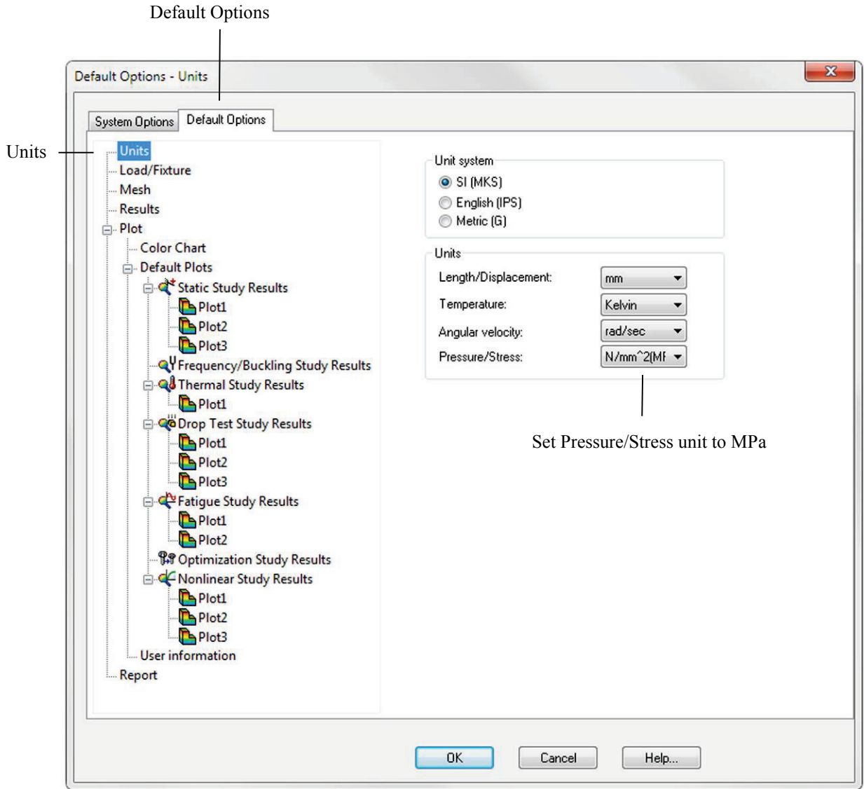
Figure 2-5: Simulation Options window.
