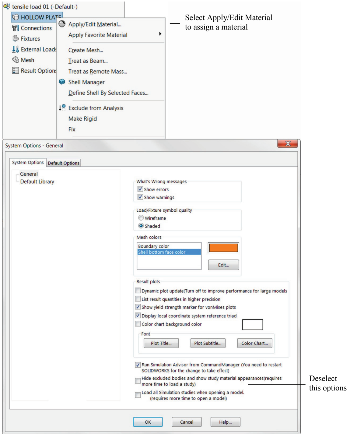
Figure 2-8: Assigning material properties.
