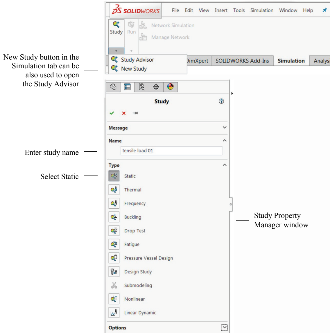
Figure 2-6: Creating a new study.
