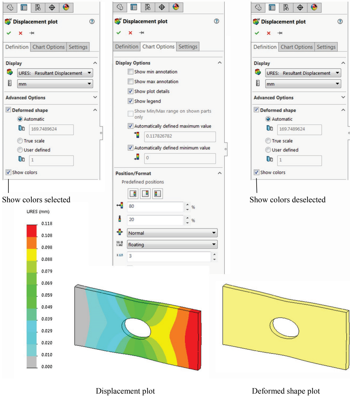
Figure 2-26: Displacement plot (left) and Deformation plot (right).
