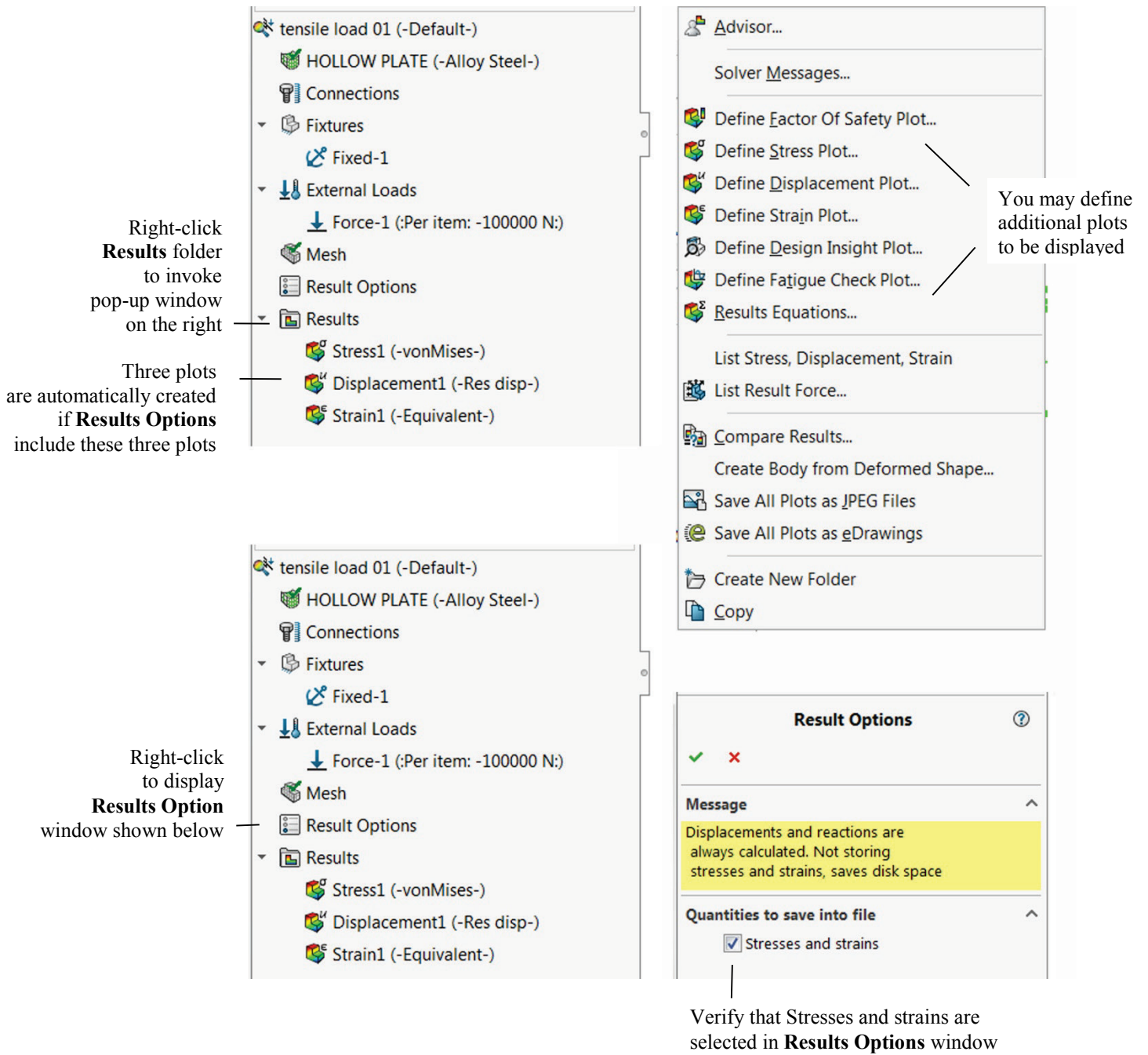
Figure 2-22: More plots and folders can be added to the Results folder.
