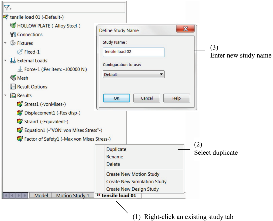
Figure 2-33: A study can be copied into another study in three steps as shown.
