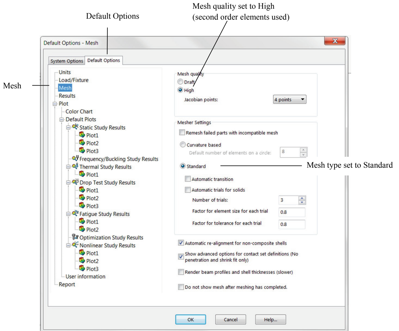
Figure 2-13: Mesh settings in the Options window.
