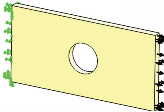
Figure 2-37: Two methods of defining prescribed displacement.
