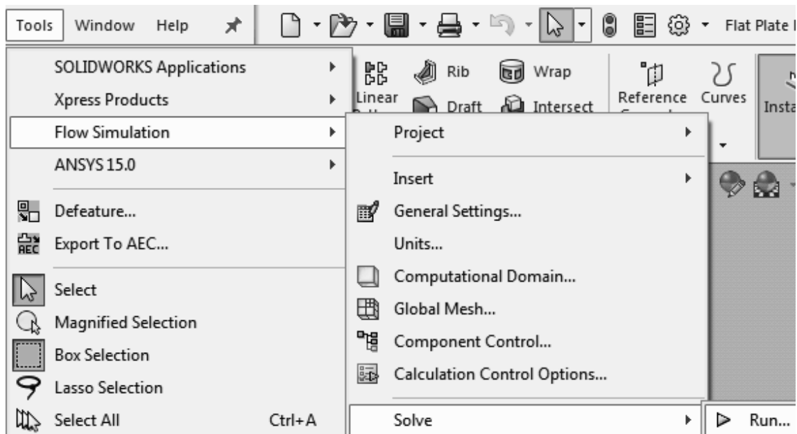
Figure 2.22a) Starting calculations
