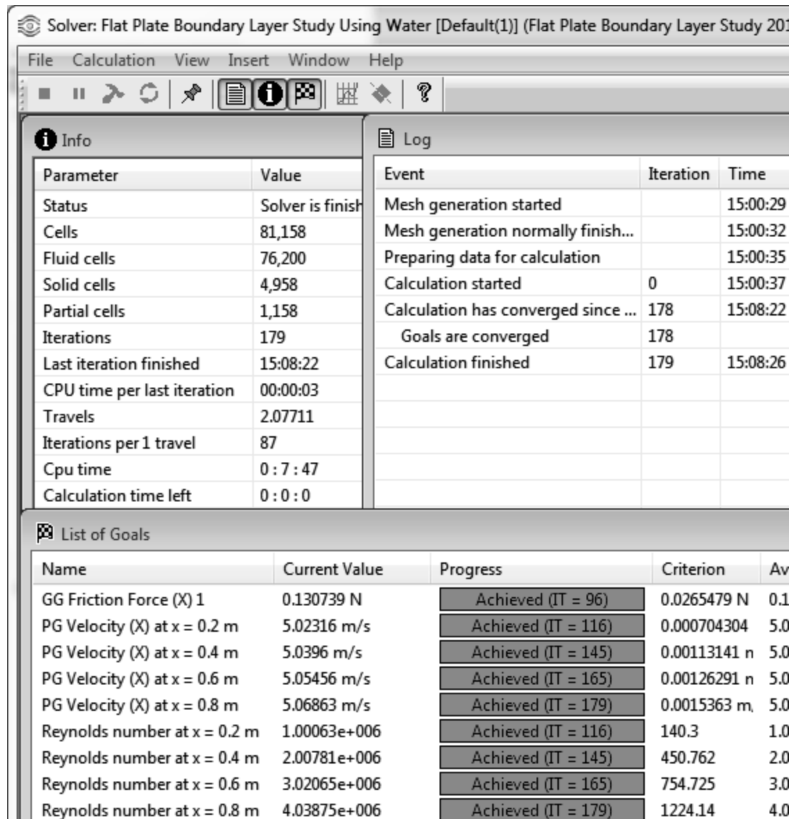
Figure 2.29d) Solver window and goals table for calculations of turbulent boundary layer
