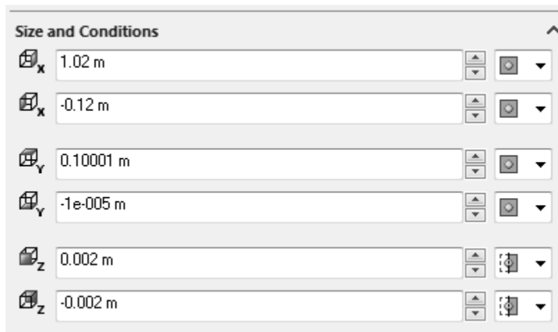
Figure 2.28a) Setting the size of the computational domain
