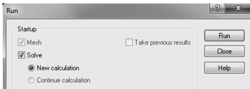
Figure 2.22b) Run window
