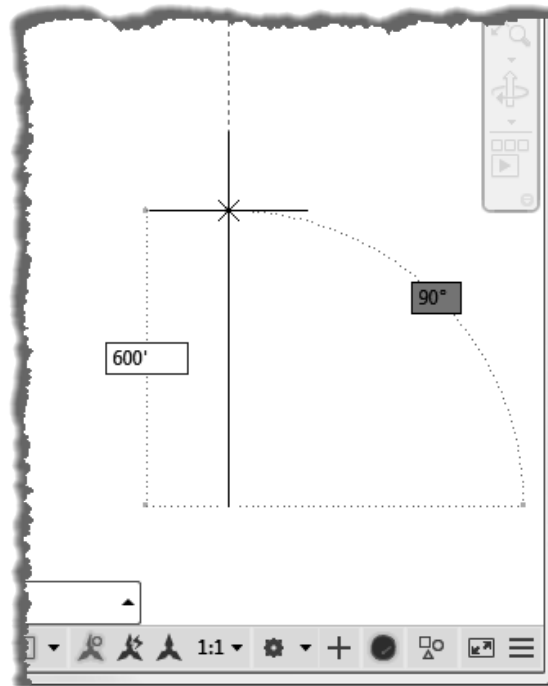
FIGURE 2-1.11 Drawing another line with the help of Polar Tracking
