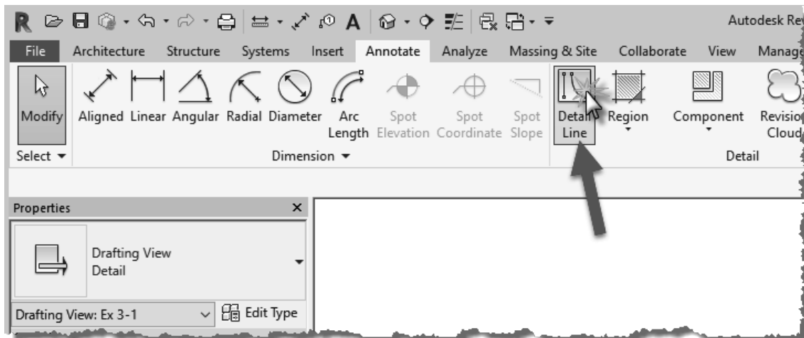
FIGURE 3-1.5 Annotate tab
