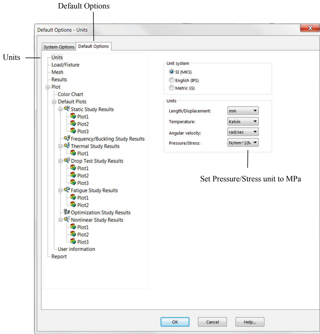
Figure 2-5: Simulation Options window.
