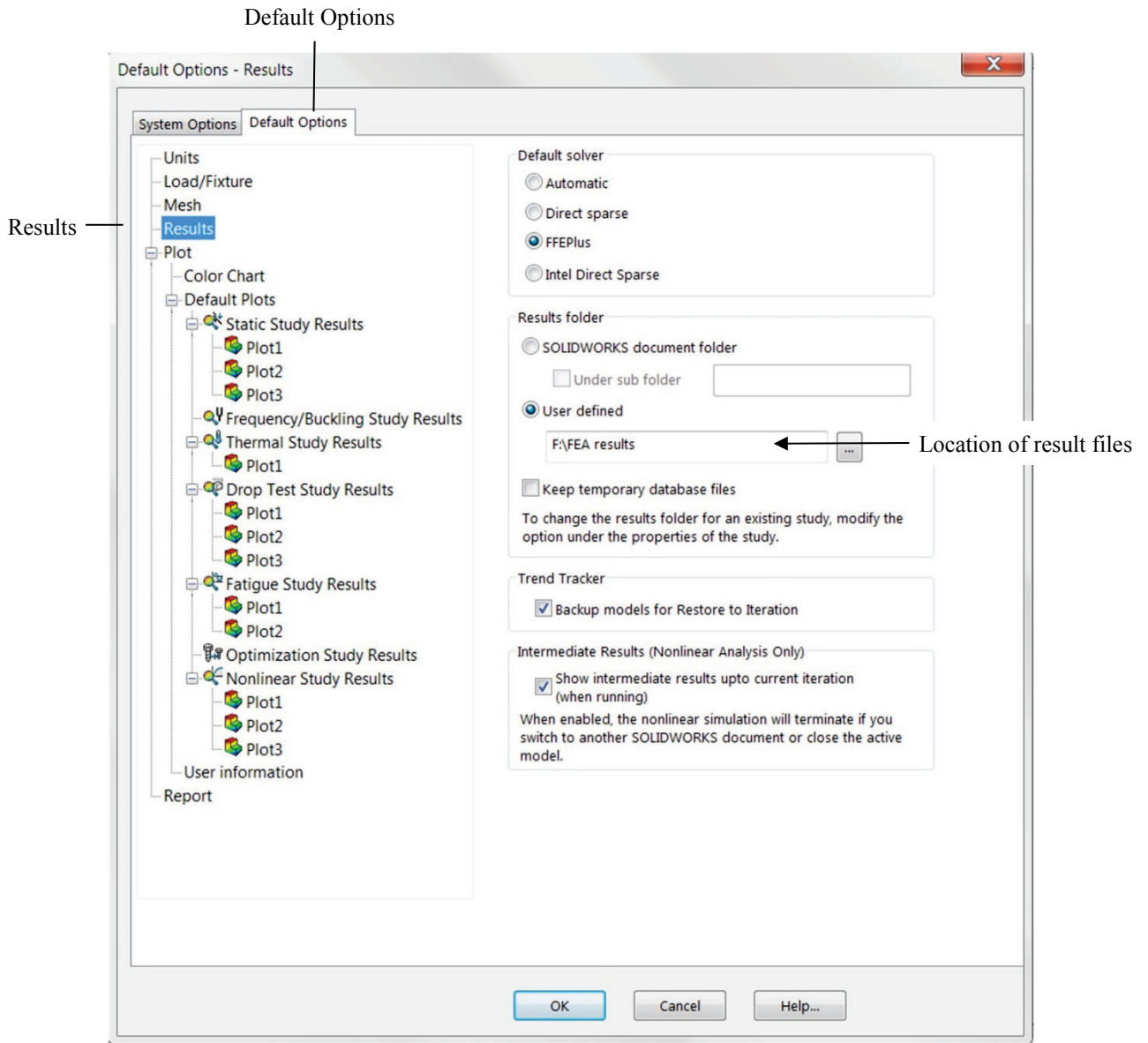
Figure 2-41: Location of solution database files.
