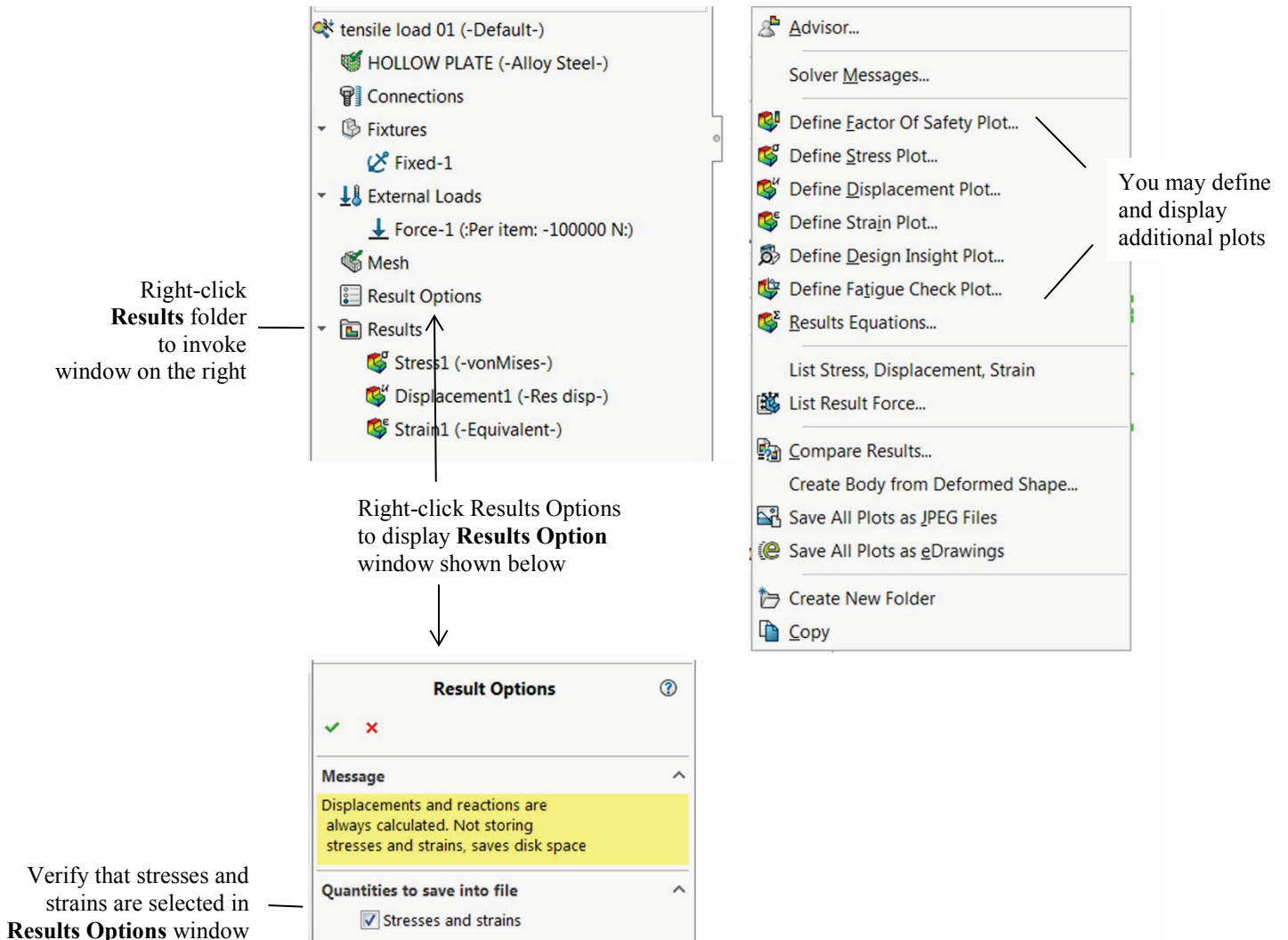
Figure 2-22: More plots and folders can be added to the Results folder.
