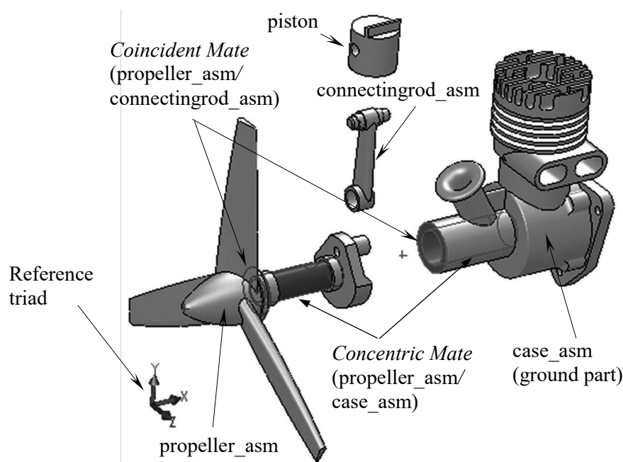
Figure 1-12 Assembly Mates Defined for the Engine Model (Explode View)
