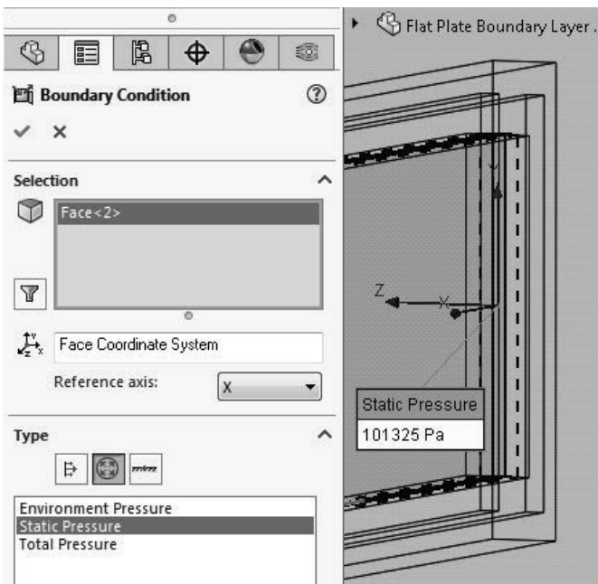
Figure 2.18a) Selection of static pressure as boundary condition at the outlet of the flow region
