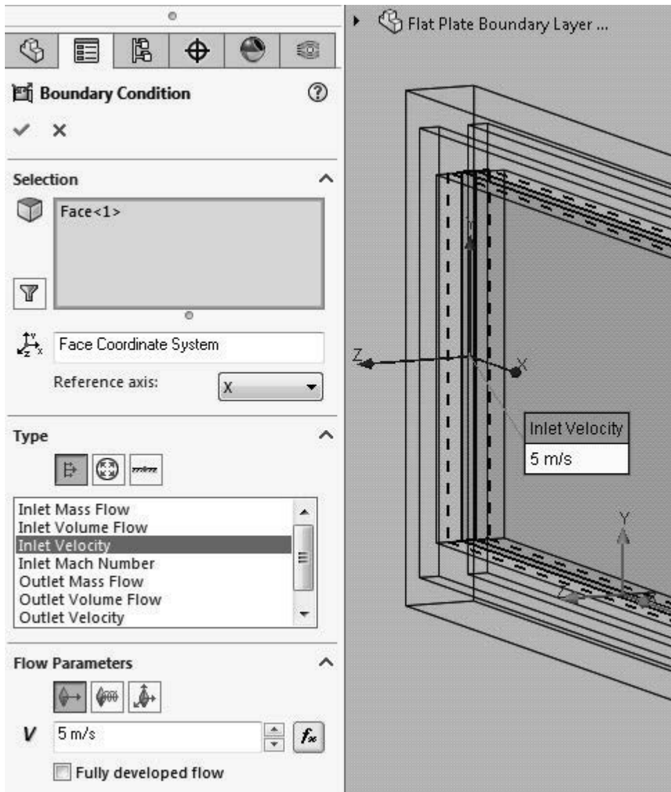
Figure 2.17c) Velocity boundary condition on the inflow
