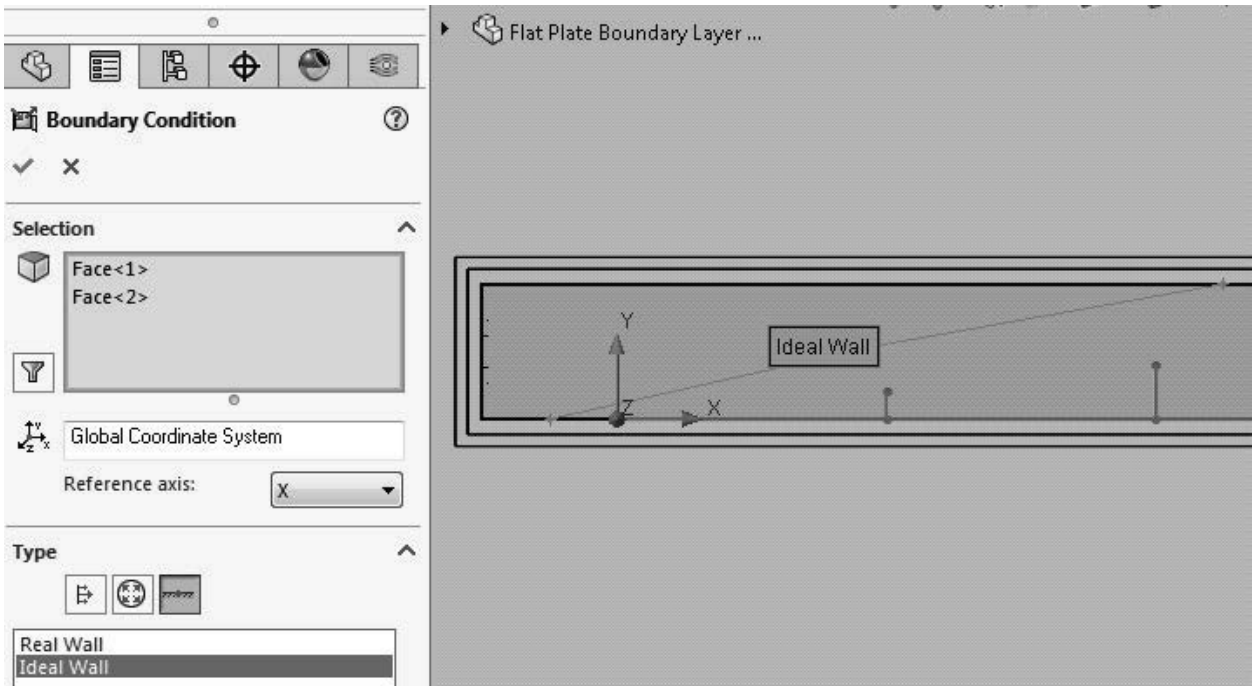
Figure 2.19 Ideal wall boundary condition for two wall sections
