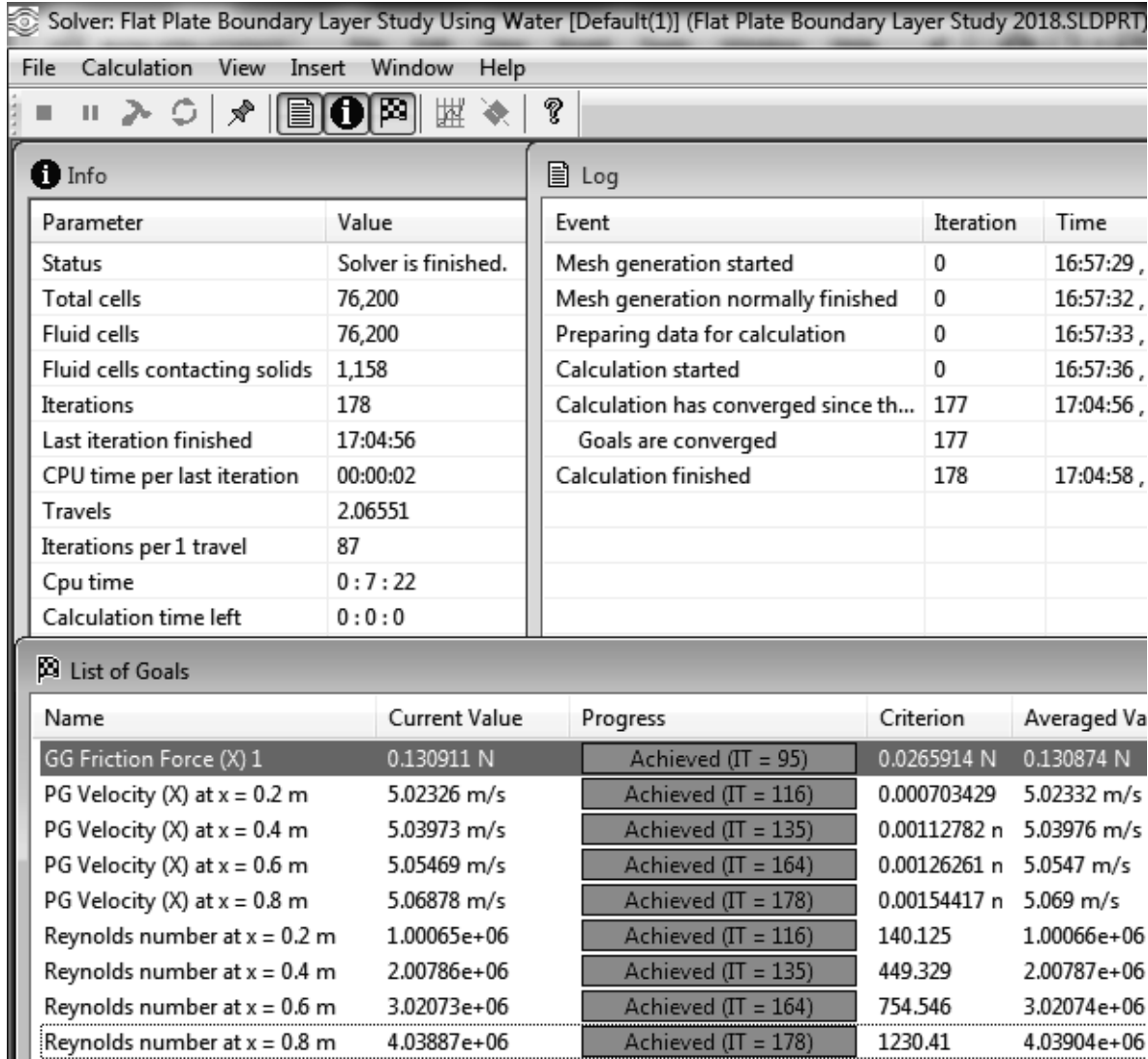
Figure 2.29d) Solver window and goals table for calculations of turbulent boundary layer
