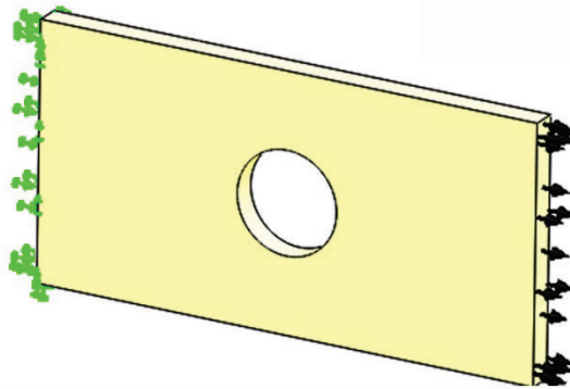
Figure 2-37: Two methods of defining prescribed displacement.
