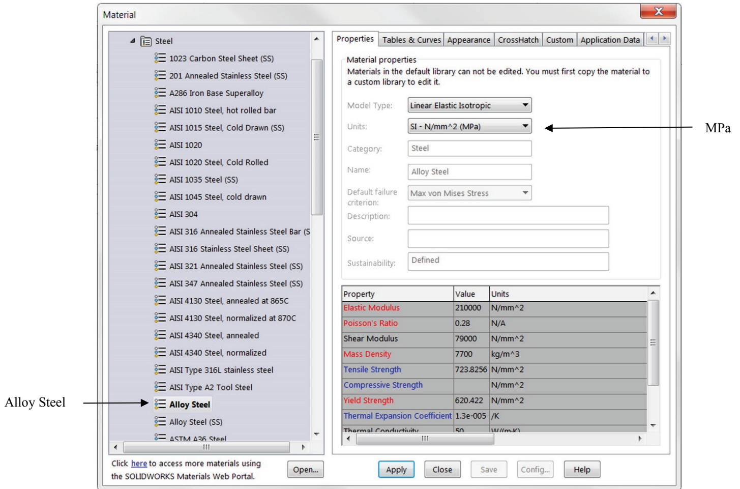
Figure 2-9: Material window.
