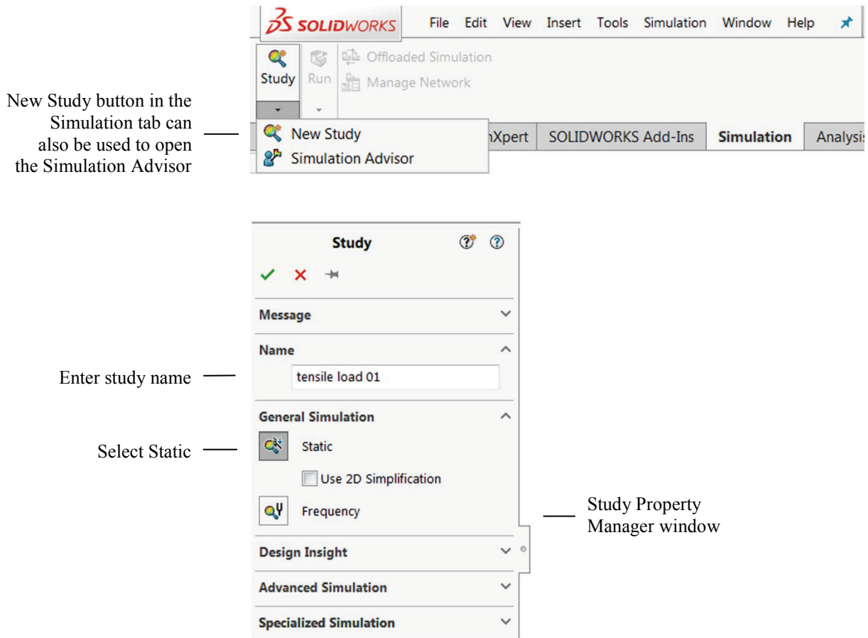
Figure 2-6: Creating a new study.
