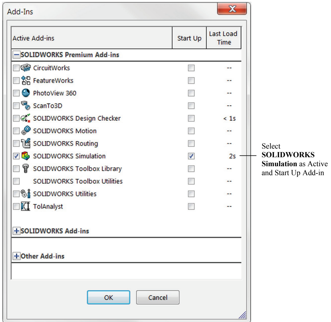
Figure 2-2: Add-Ins list in SOLIDWORKS.
