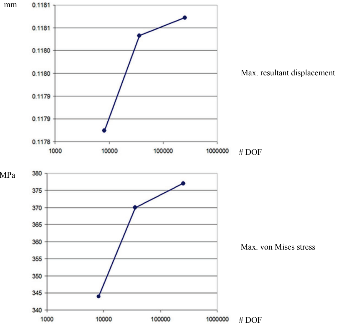
Figure 2-36: Maximum resultant displacement (top) and maximum von Mises stress (bottom).
