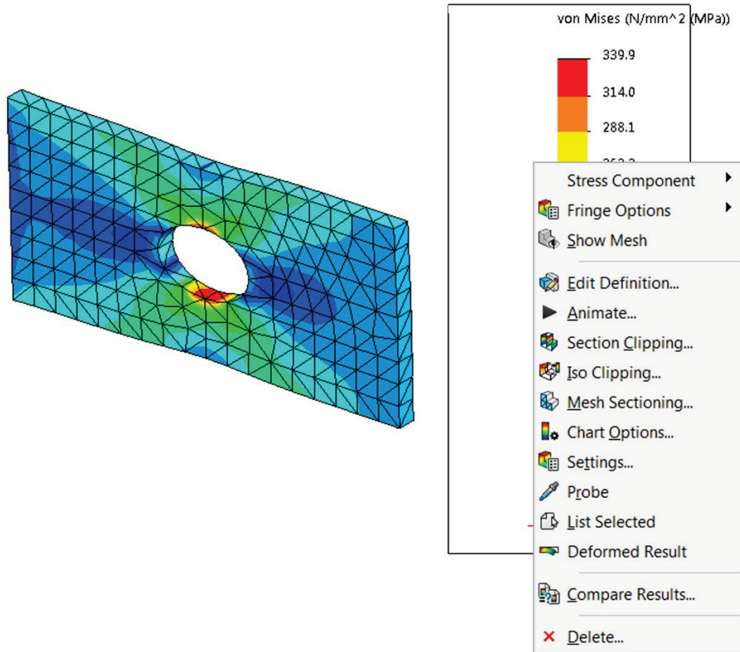
Figure 2-25: The modified stress plot is shown with discrete fringes and the mesh superimposed on the stress plot (top). Numbers use floating format with one decimal place. The plot also shows a shortcut menu that can be used to modify display options.
