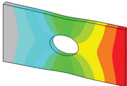
Displacement plot
