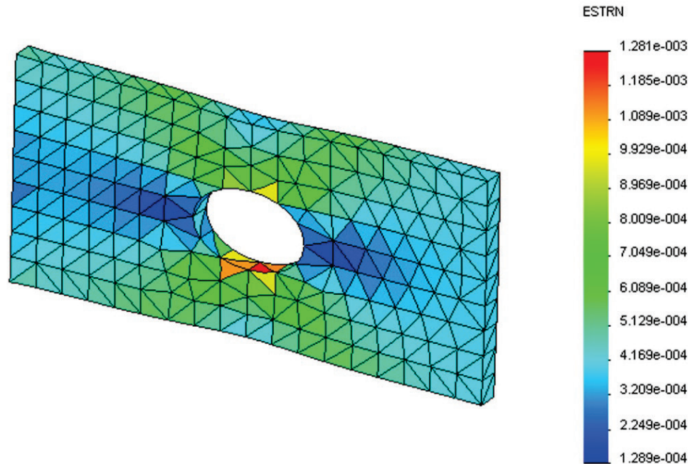
Figure 2-27: Strain results.
