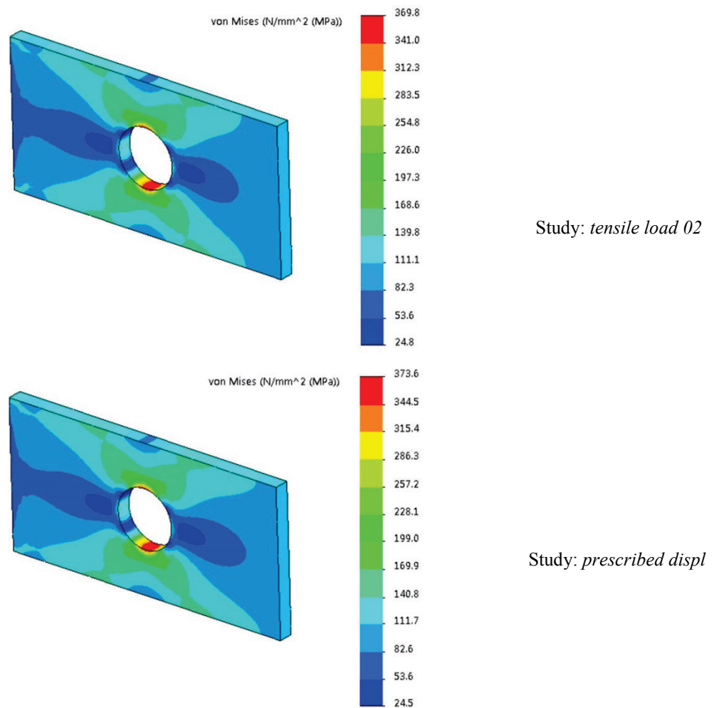
Figure 2-38: Comparison of von Mises stress results.
