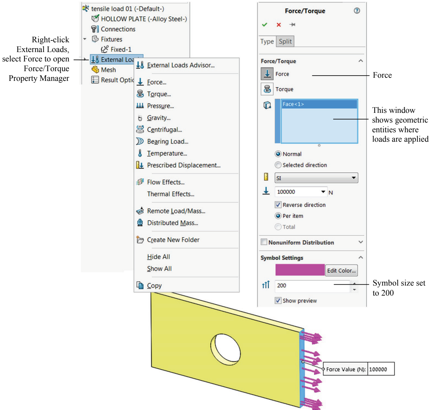
Figure 2-11: Pop-up menu for the External Loads folder and Force window.
