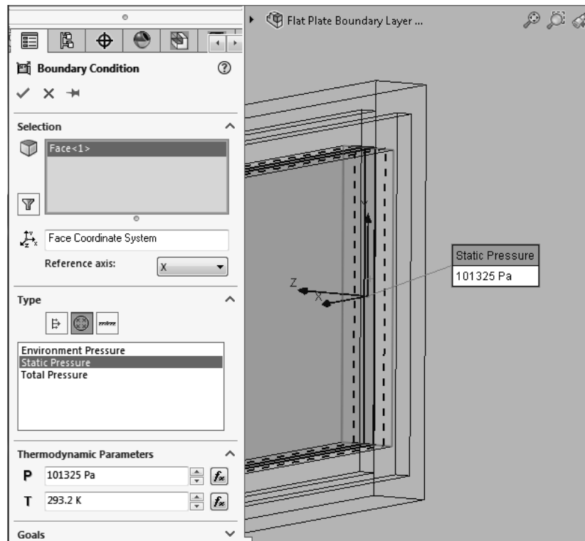
Figure 2.18a) Selection of static pressure as boundary condition at the outlet of the flow region
