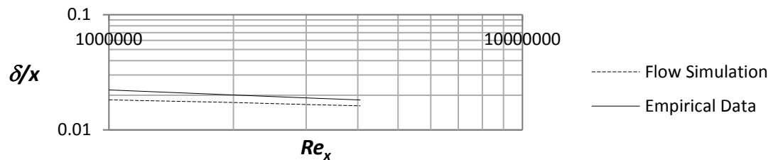
Figure 2.30b) Boundary layer thickness for turbulent boundary layers at Re_x = 10^6 - 4.04 \cdot 10^6
