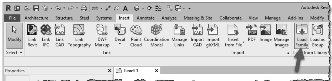
FIGURE 3-5.1 Load Family
