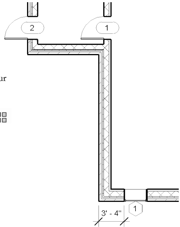
FIGURE 3-5.9 Exterior window
