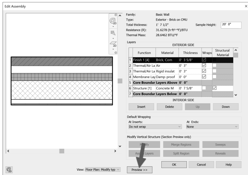
FIGURE 3-2.5 Edit Assembly
