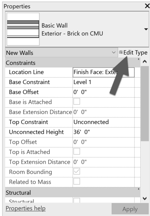
FIGURE 3-2.3 Properties Palette
