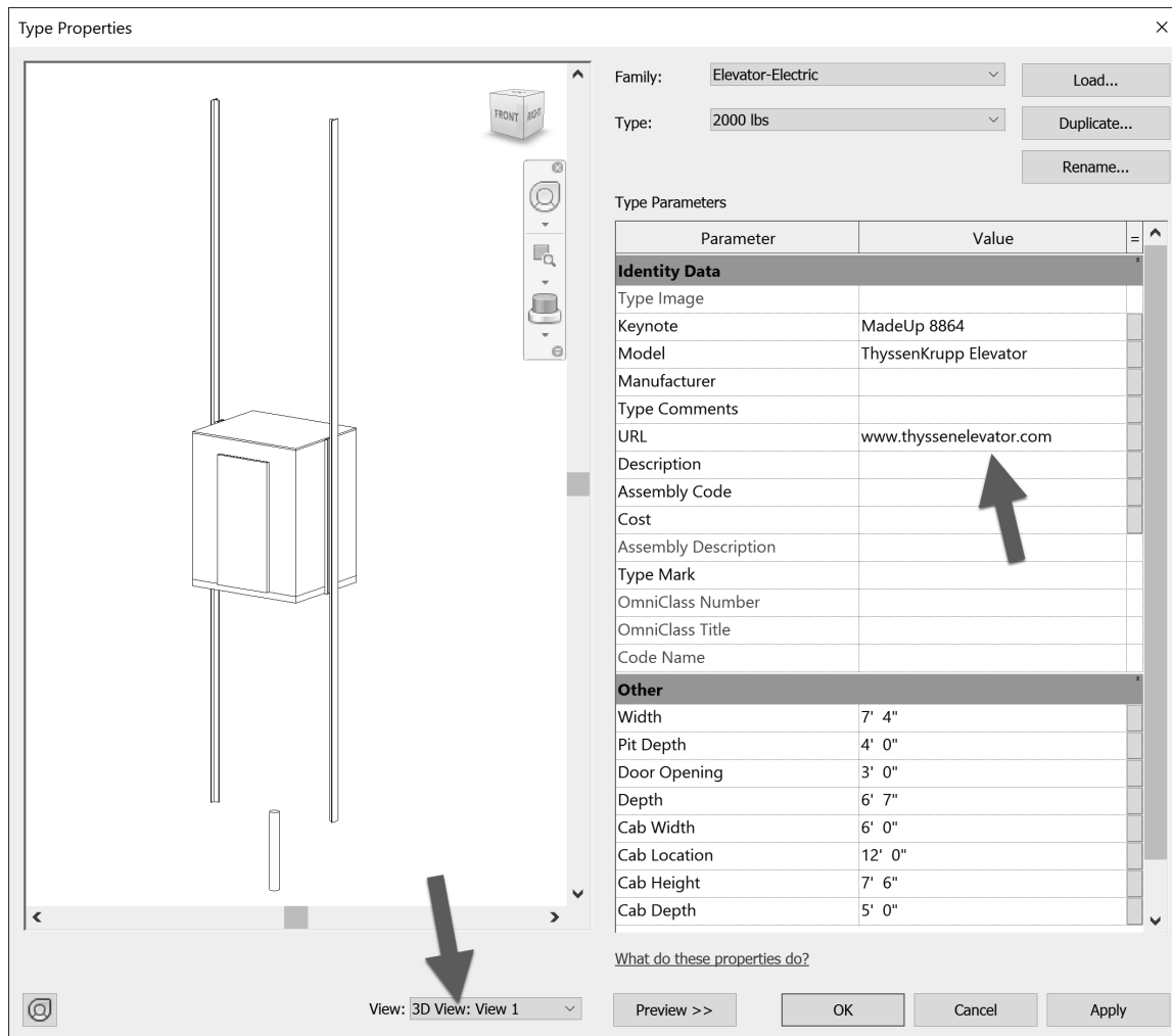
FIGURE 3-4.2 Elevator properties
