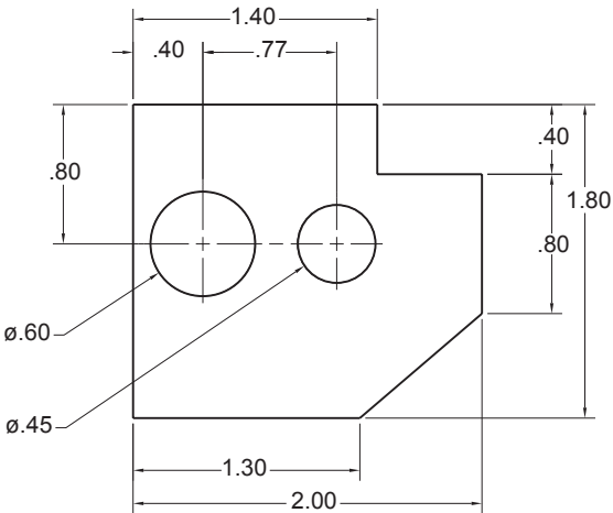
Exercise 2.2 Gasket
