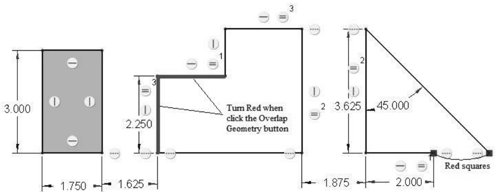
Figure 3-9 Sketched Sections
