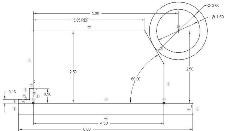
Figure 3-63 Jig Design 1b
