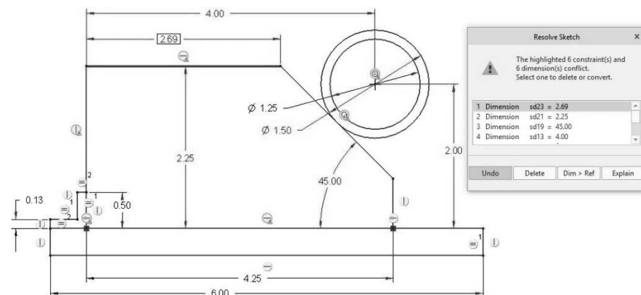
Figure 3-56 Resolve Sketch
