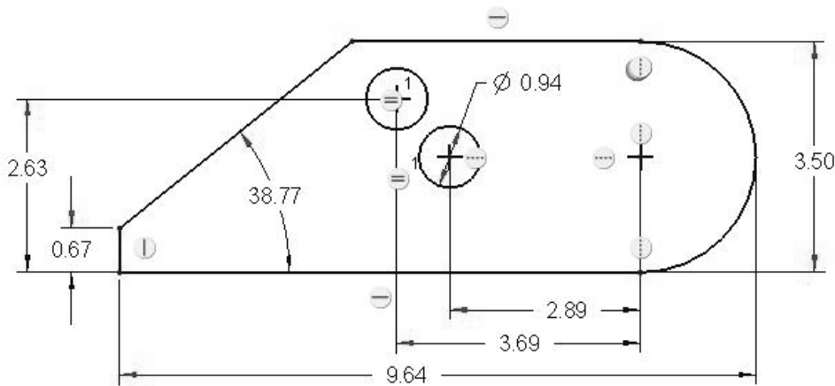
Figure 3-22 Add Dimensions
