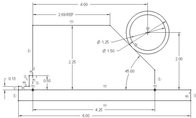
Figure 3-45 Layout 1
