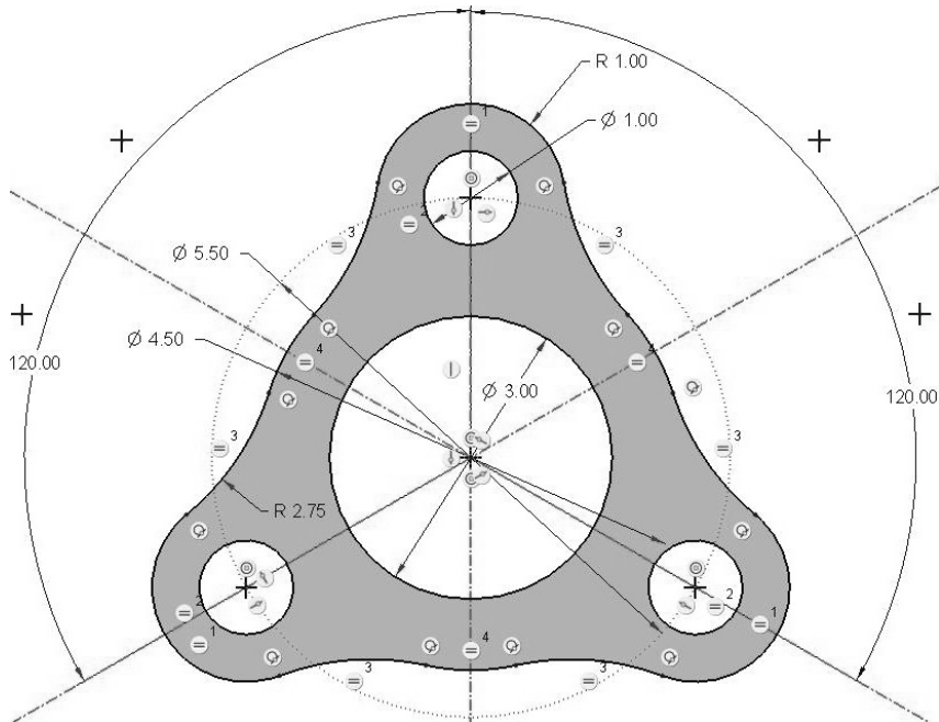
Figure 3-79 Problem 10—Cork Gasket
