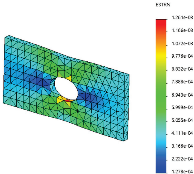
Figure 2-27: Strain plot.
