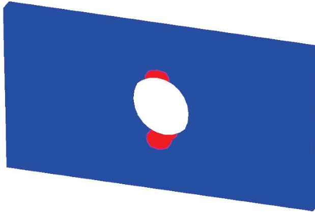
Figure 2-29: The red color displays the areas where the factor of safety is below 3. Irregular shape of red areas is caused by the coarse mesh used in this study.
