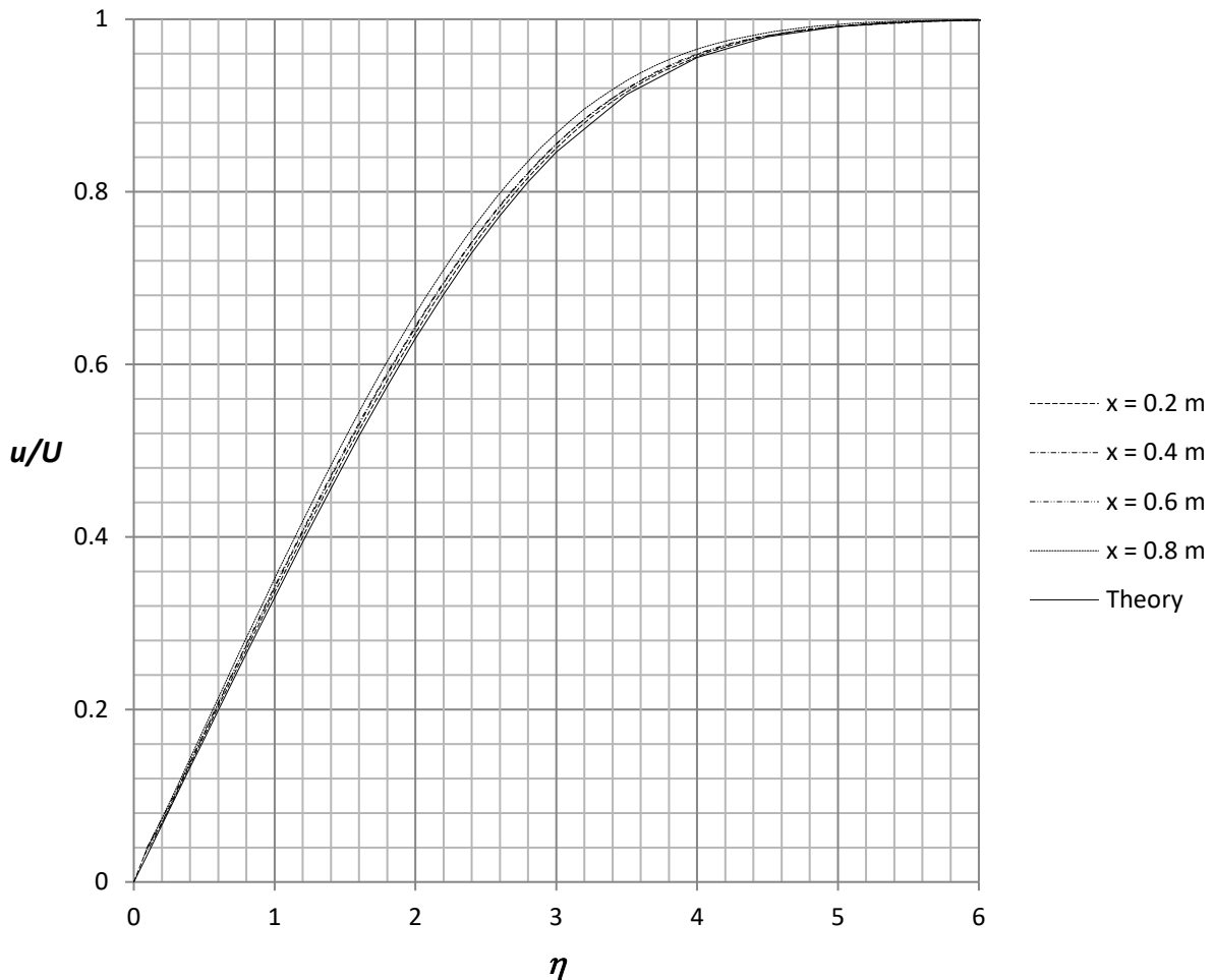
Figure 2.25a) Velocity profiles in comparison with the theoretical Blasius profile (full line)
