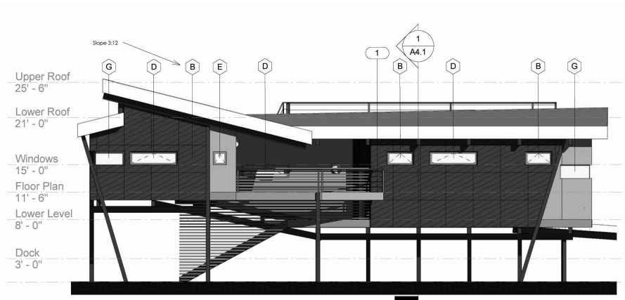
1.3 Elevation View of a Custom Home Created with 3D Modeling Software (Image courtesy of David Naumann)
