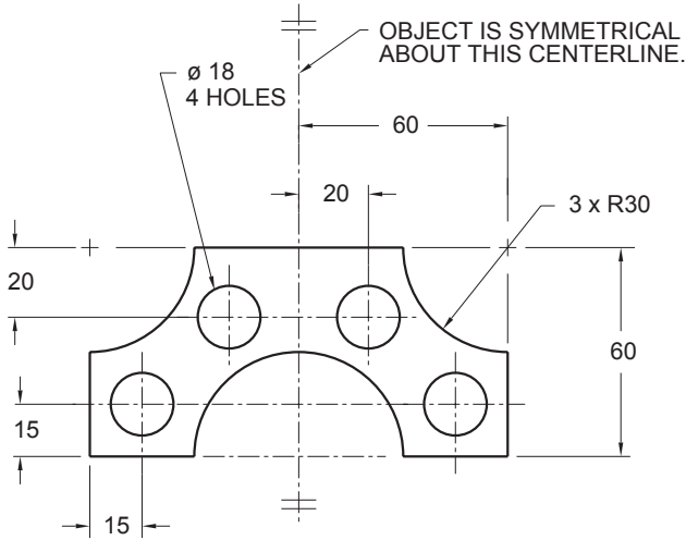
Exercise 2.1M Bracket
