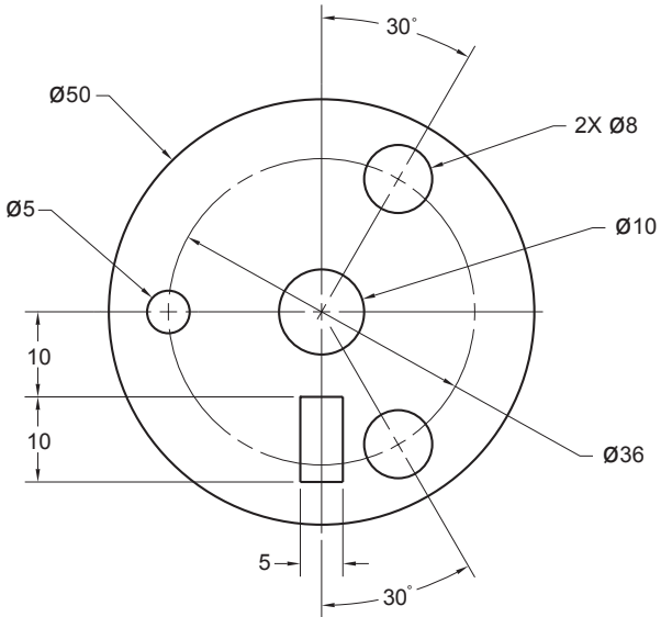
Exercise 2.3M Flange
