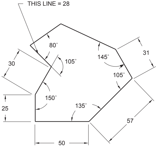
Exercise 2.4M Puzzle
