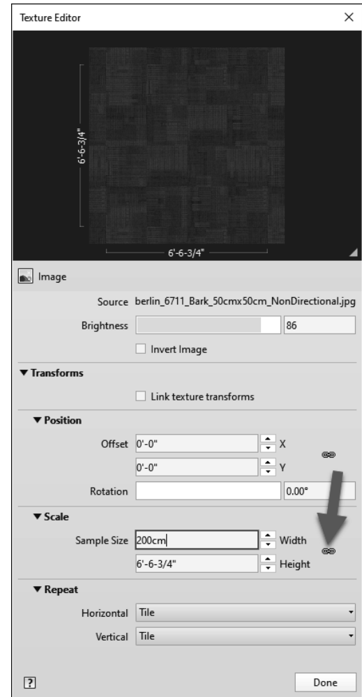
FIGURE 4-3.10 Texture Editor
