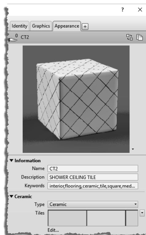
FIGURE 4-4.13 Completed CT2
