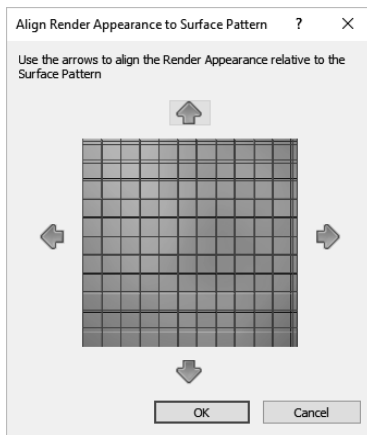
FIGURE 4-4.8 Texture alignment
