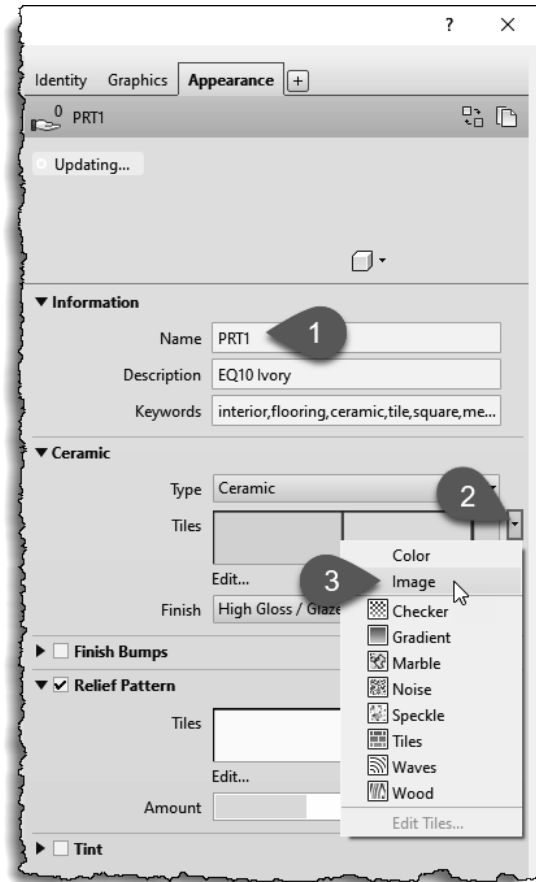
FIGURE 4-4.15 Appearance tab
