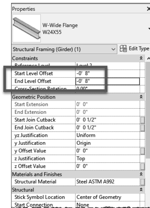
FIGURE 8-3.18 Beam properties
