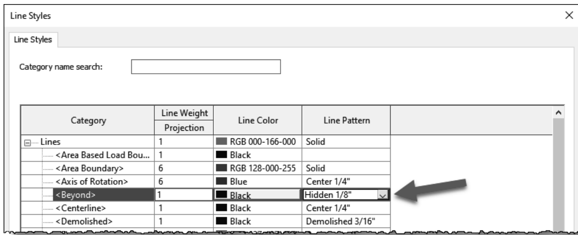
FIGURE 8-5.11 Line Style settings
