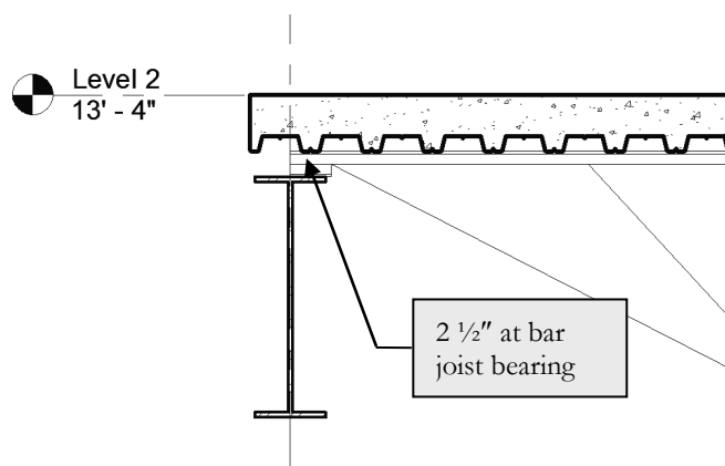
FIGURE 8-3.15 Beam supporting bar joist
