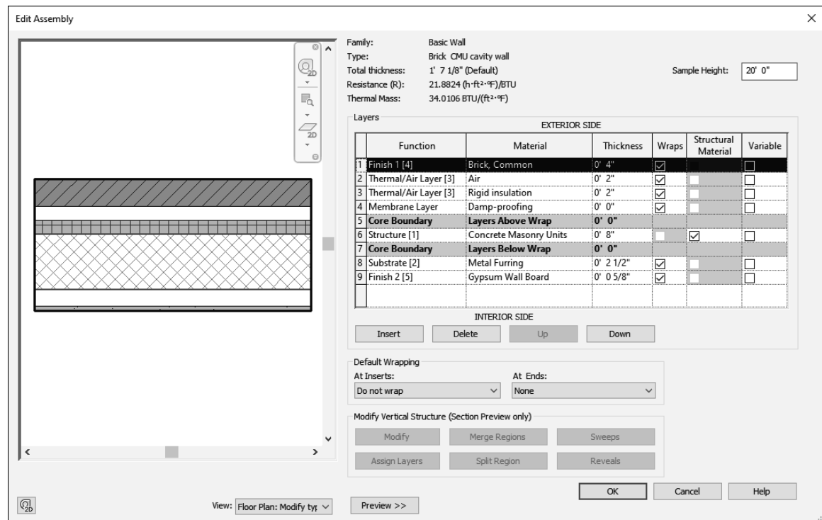
FIGURE 3-2.8 Edit Assembly for new wall type
