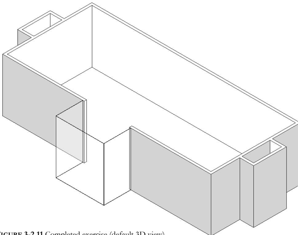
FIGURE 3-2.11 Completed exercise (default 3D view)
