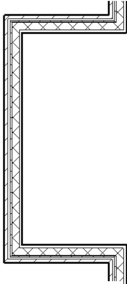
FIGURE 3-3.6 Trim tool
