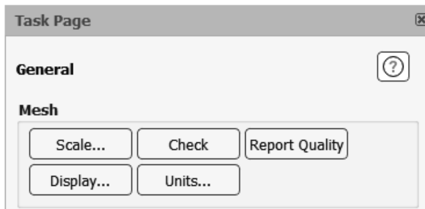
Figure 2.7a) Scale Check
