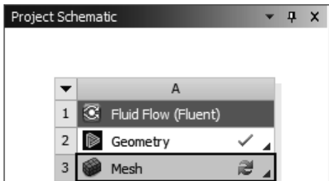
Figure 2.5a) Launching mesh
