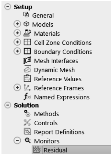
Figure 2.11a) Residual monitors
