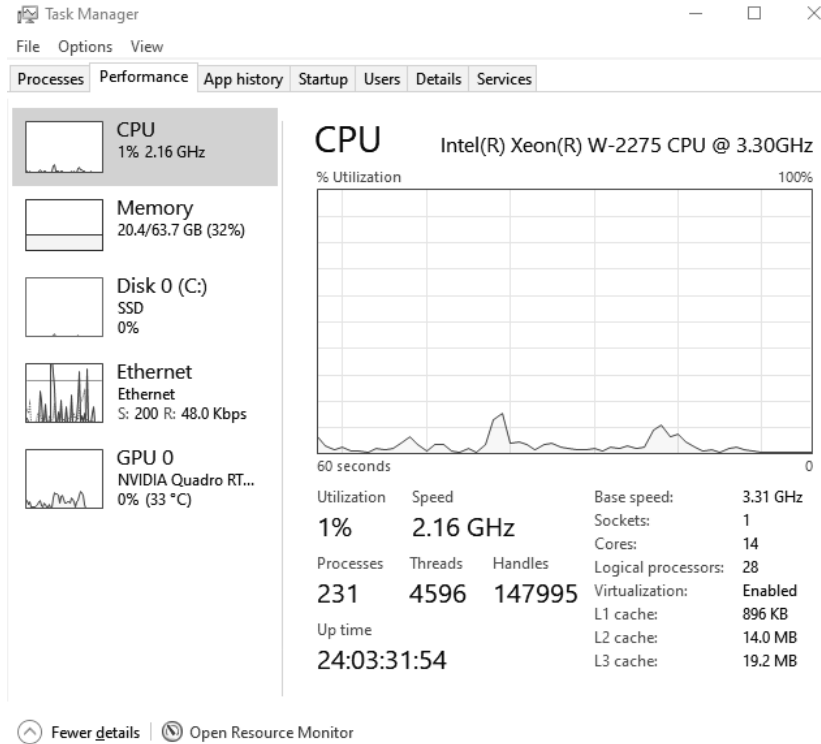
Figure 2.6b) Taskmanager
