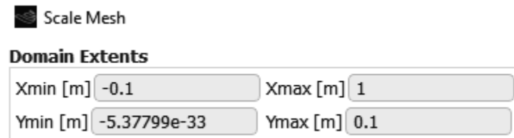
Figure 2.7b) Scale Mesh
