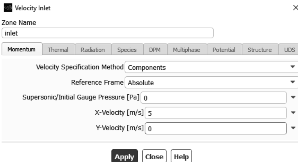
Figure 2.8c) Inlet velocity
