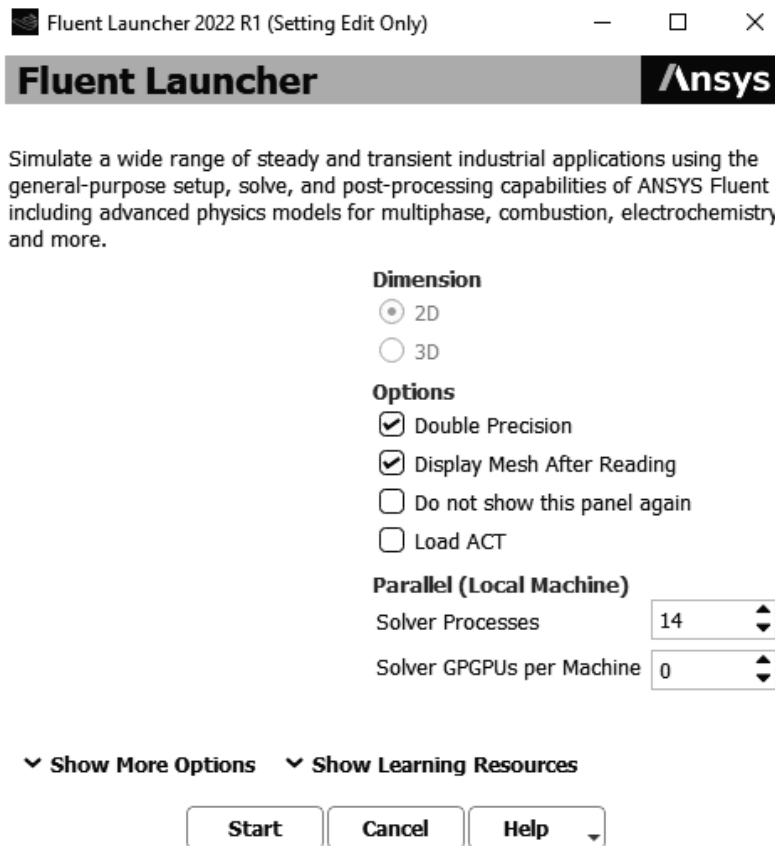
Figure 2.6c) Fluent Launcher
