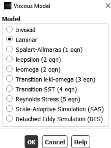
Figure 2.8a) Viscous model
