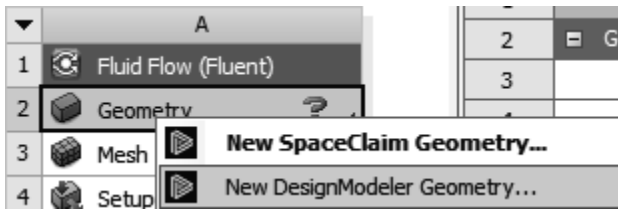
Figure 2.2b) Launching DesignModeler
