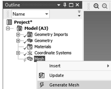
Figure 2.5b) Generating mesh
