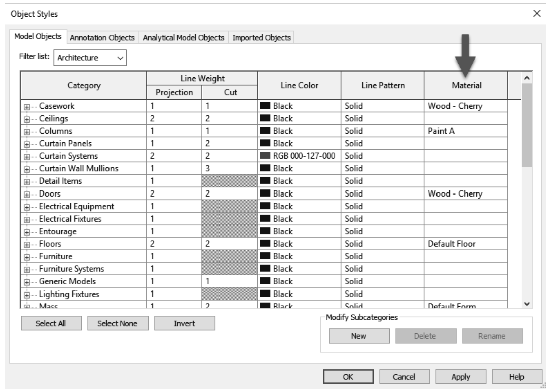
FIGURE 4-1.1 Object Styles dialog
