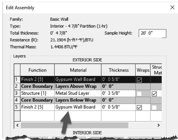
FIGURE 4-1.2 Edit Assembly dialog
