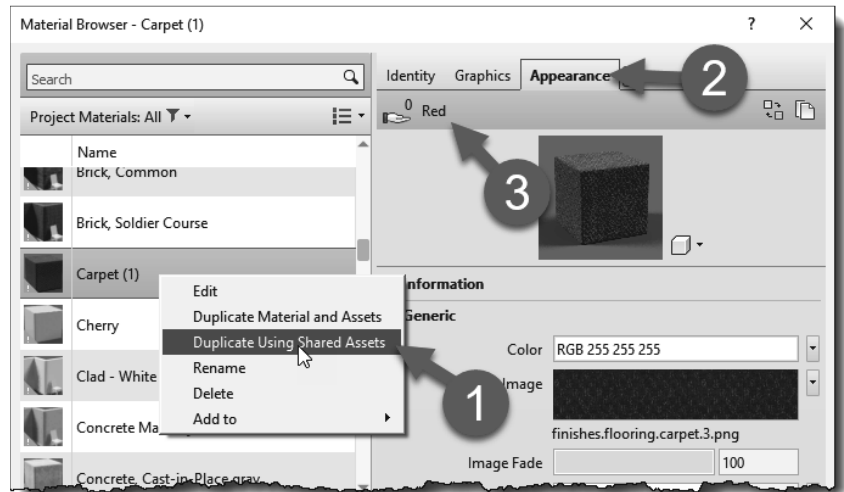
FIGURE 4-2.18 Duplicating a material
