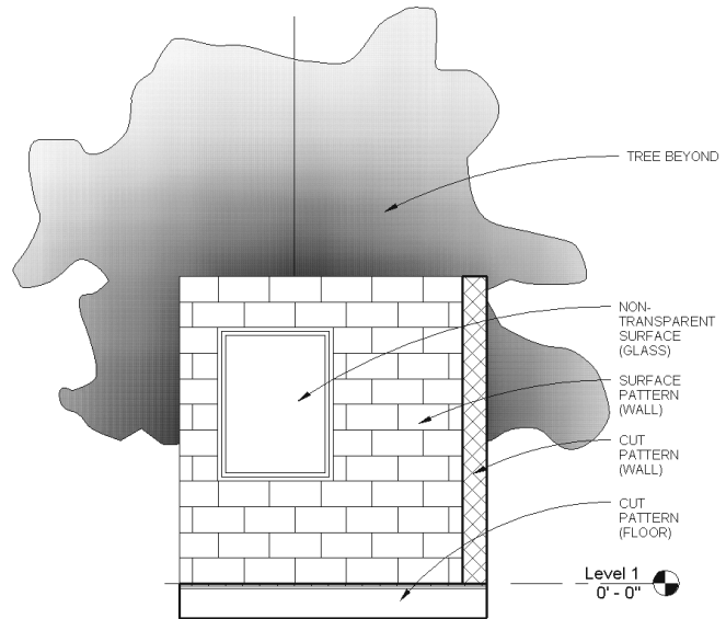
ELEVATION / SECTION VIEW
