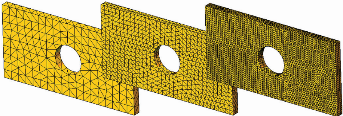
Figure 2-30: Coarse, medium, and fine meshes. Three meshes used to study the effects of element size on results.
