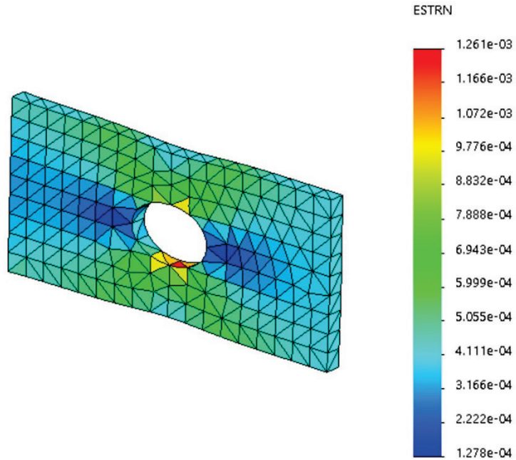
Figure 2-27: Strain plot.
