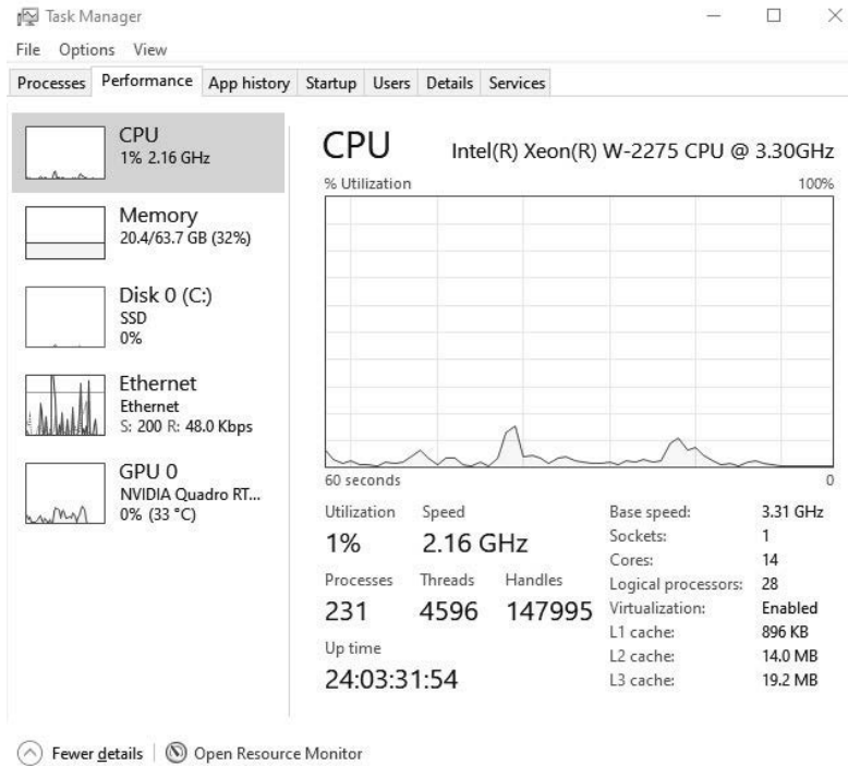
Figure 2.6b) Taskmanager
