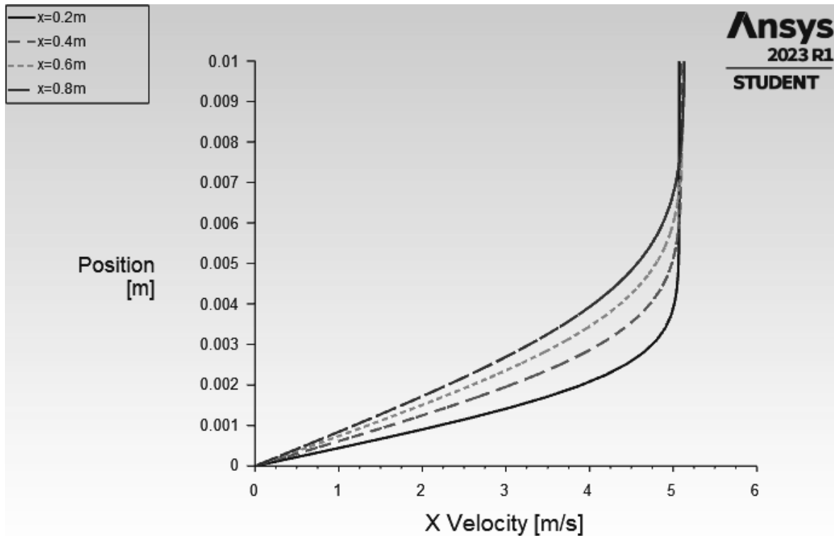
Figure 2.16b) Velocity profiles for a laminar boundary layer on a flat plate
