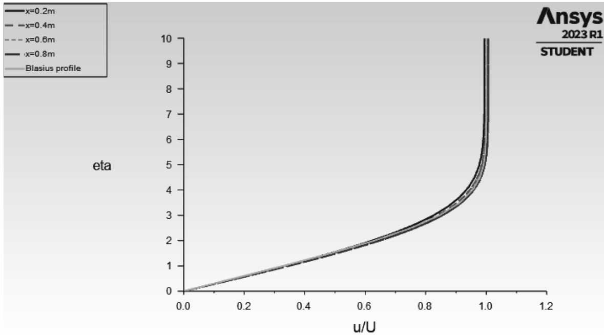
Figure 2.17d) Self-similar velocity profiles for a laminar boundary layer on a flat plate
