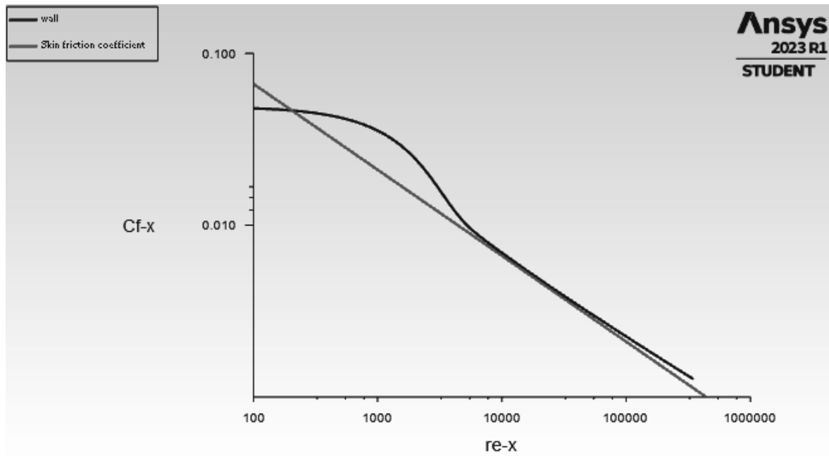
Figure 2.18d) Comparison between Ansys Fluent and theoretical skin friction coefficient for laminar boundary layer flow on a flat plate
