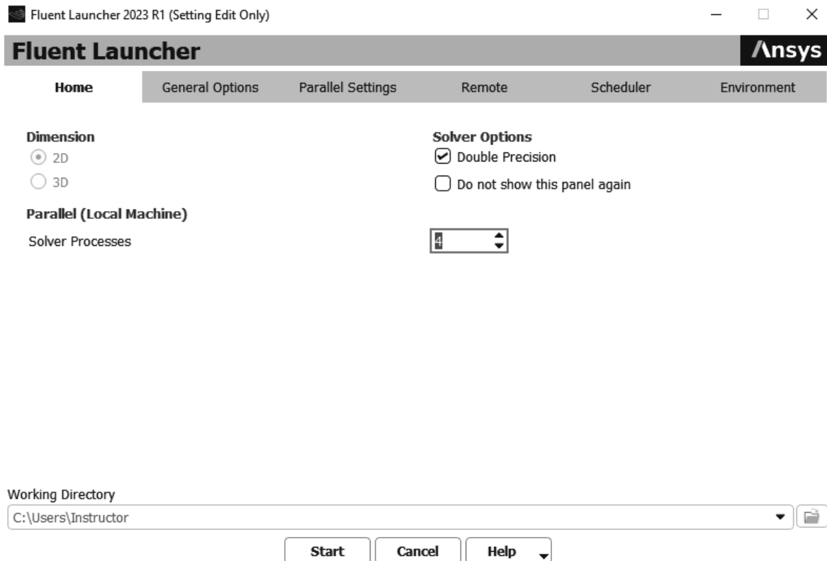
Figure 2.6c) Fluent Launcher
