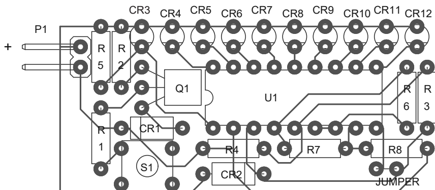
1.7 Detail of Printed Circuit Board Prepared from the Schematic Shown in Figure 1.7
