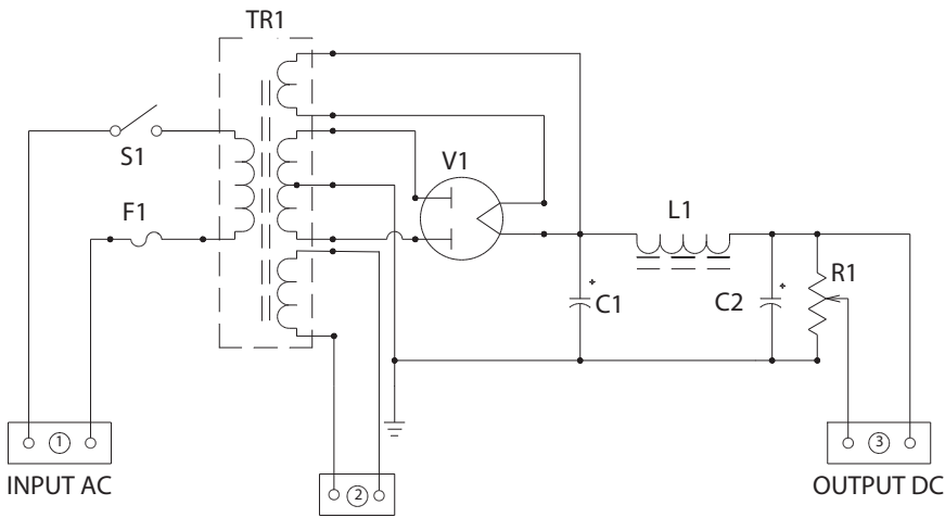
POWER SUPPLY
