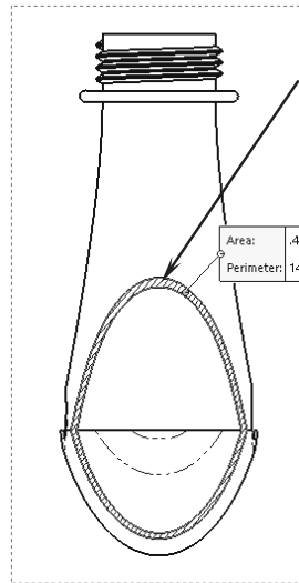
SECTION B-B
