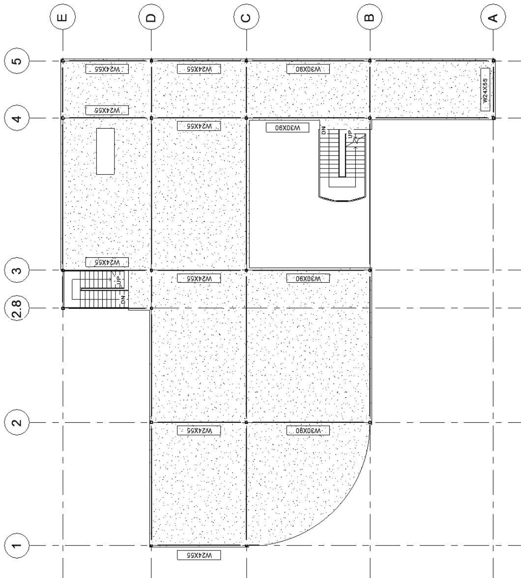
FIGURE 8-3.21 Level 2 beams with tops 5 1/2" below the Level 2 plane; image rotated to increase size, and the beam tags have been temporarily hidden for the beams placed in the previous step.
