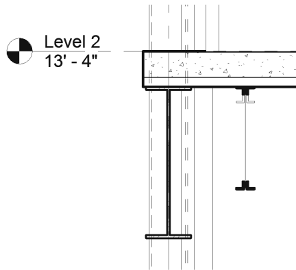
FIGURE 8-3.14 Beam parallel to bar joist
