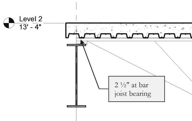
FIGURE 8-3.15 Beam supporting bar joist
