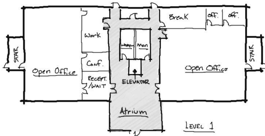
FIGURE 3-1.1 Level 1 floor plan sketch
