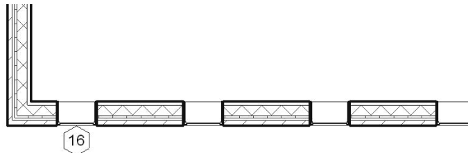
FIGURE 3-5.11 Window after array
