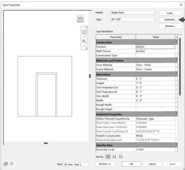
FIGURE 3-5.6 Door type properties
