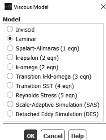
Figure 2.8a) Viscous model
