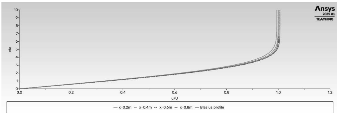
Figure 2.17d) Self-similar velocity profiles for a laminar boundary layer on a flat plate
