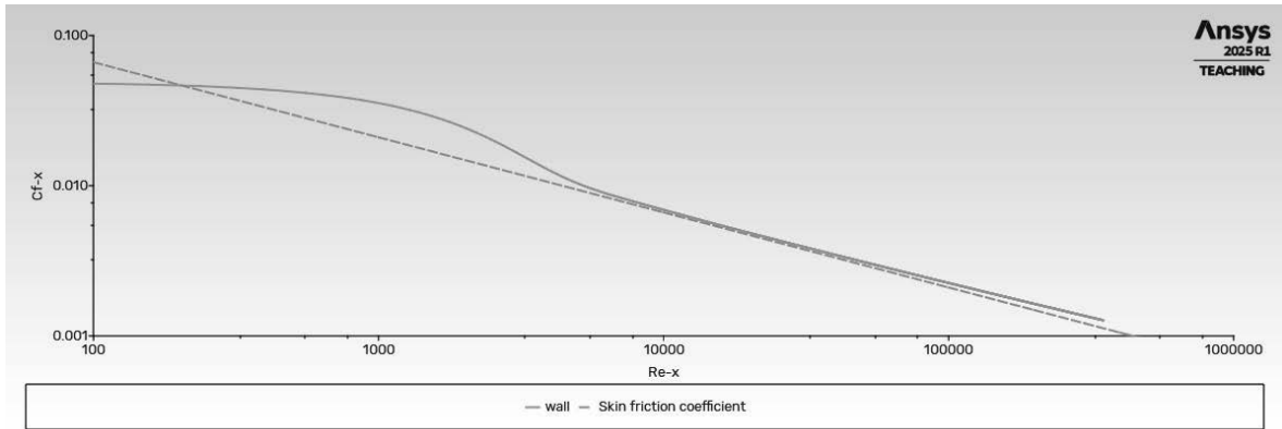
Figure 2.18d) Comparison between Ansys Fluent and theoretical skin friction coefficient for laminar boundary layer flow on a flat plate
