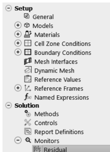
Figure 2.11a) Residual monitors
