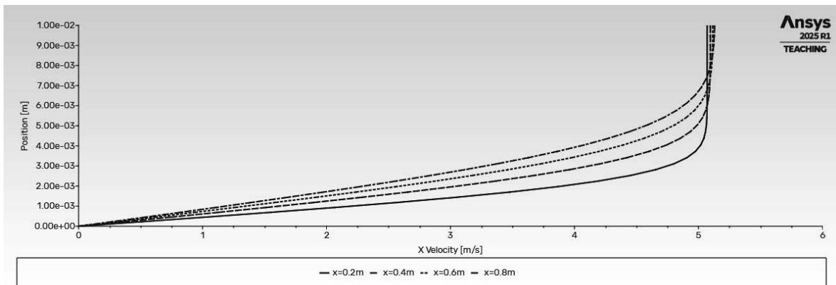
Figure 2.16b) Velocity profiles for a laminar boundary layer on a flat plate
