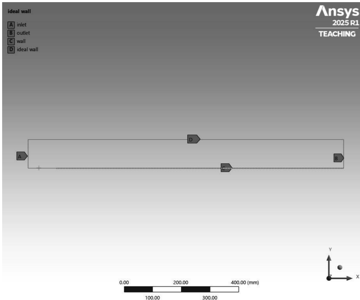
Figure 2.5i) Named selections
