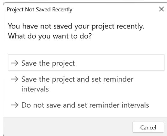
FIGURE 3-2.6 Save reminder
