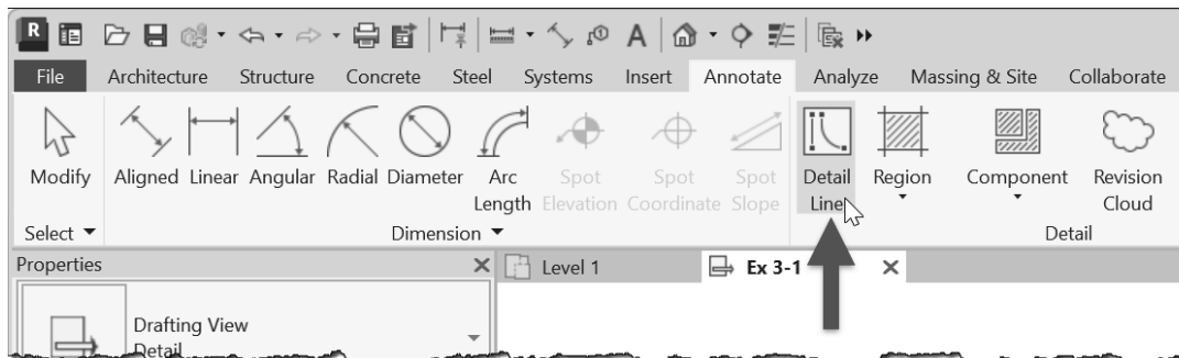
FIGURE 3-1.5 Annotate tab
