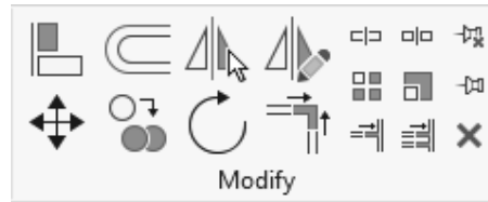
FIGURE 3-3.1 Modify panel
