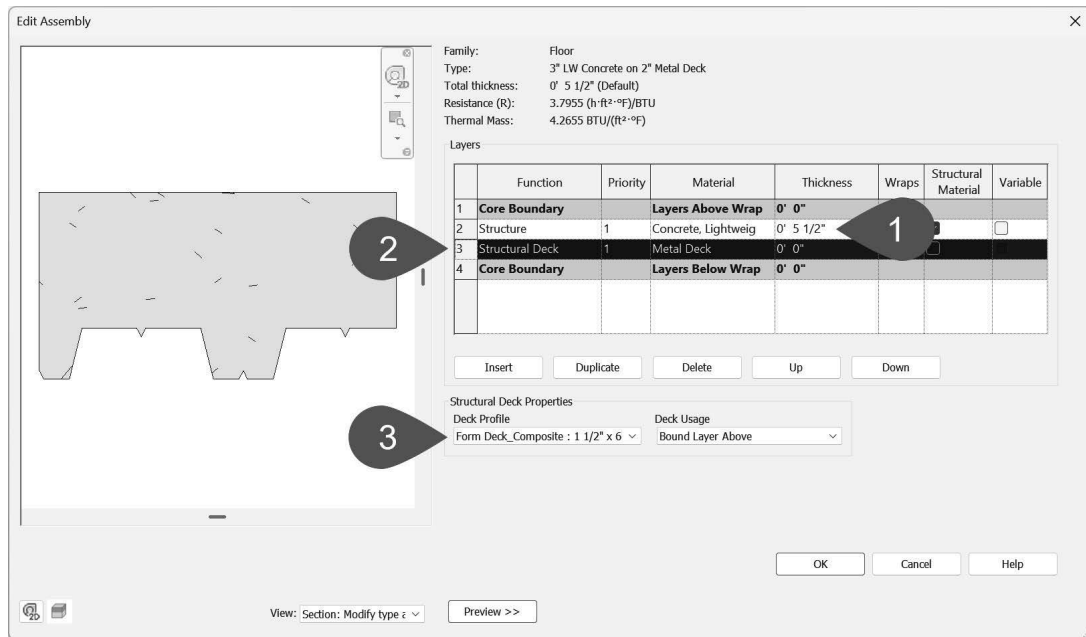
FIGURE 8-4.1 Editing the Level 2 floor construction
