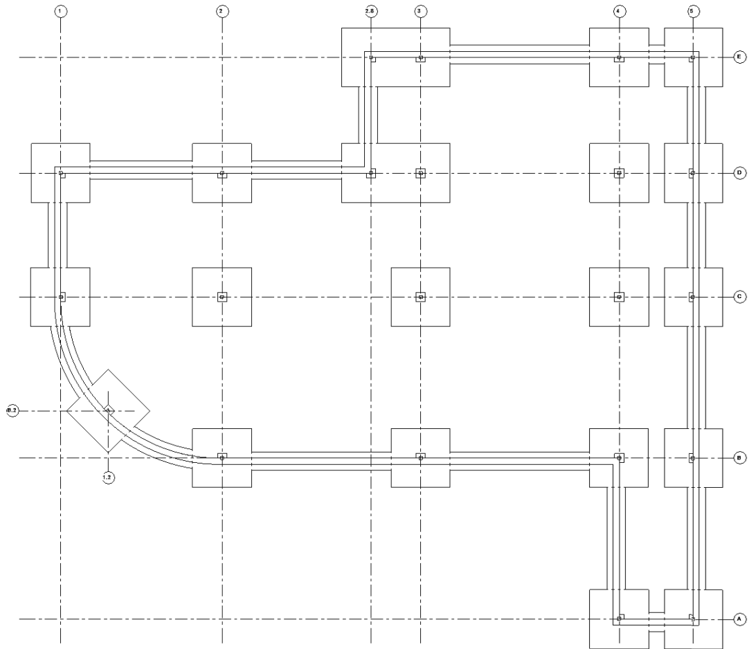
FIGURE 8-5.9 Isolated footings placed
