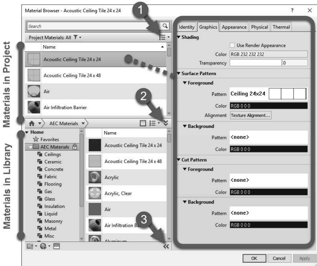
FIGURE 4-2.1 Materials dialog
