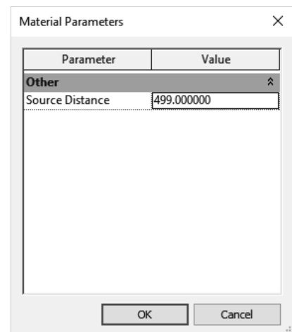
FIGURE 4-2.25 Material parameters
