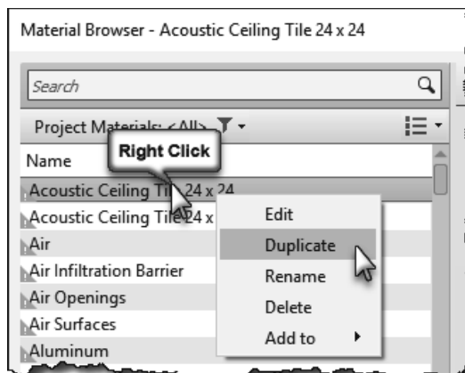
FIGURE 4-2.5 Right-click options
