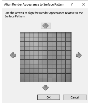
FIGURE 4-4.8 Texture alignment
