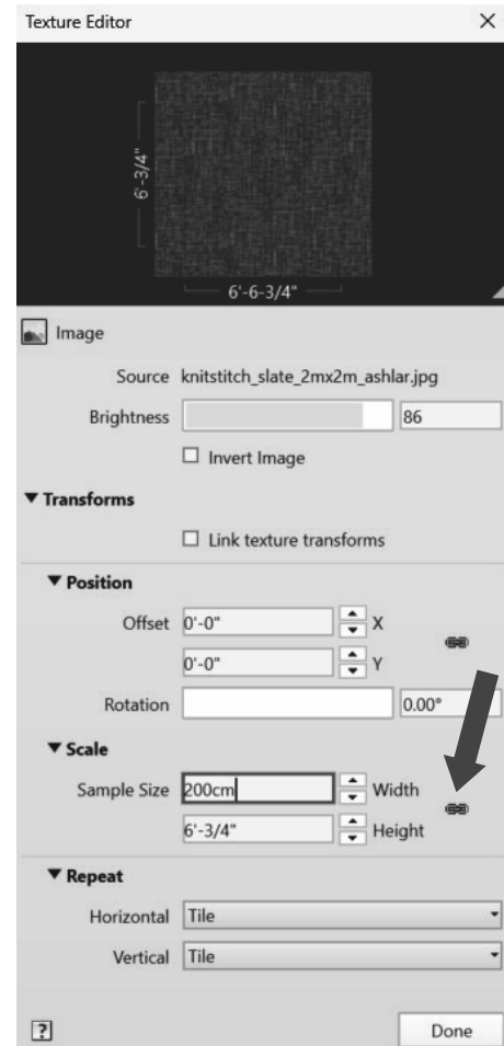
FIGURE 4-3.10 Texture Editor
