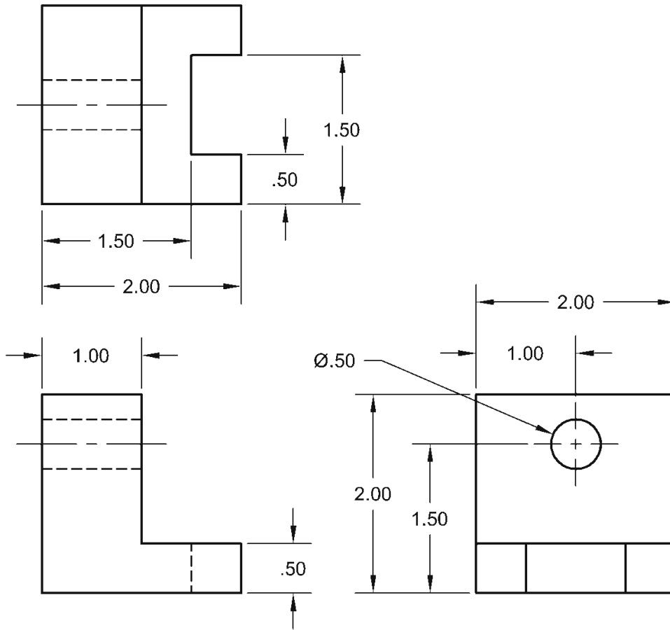
Figure 5.2-1: A typical orthographic projection
