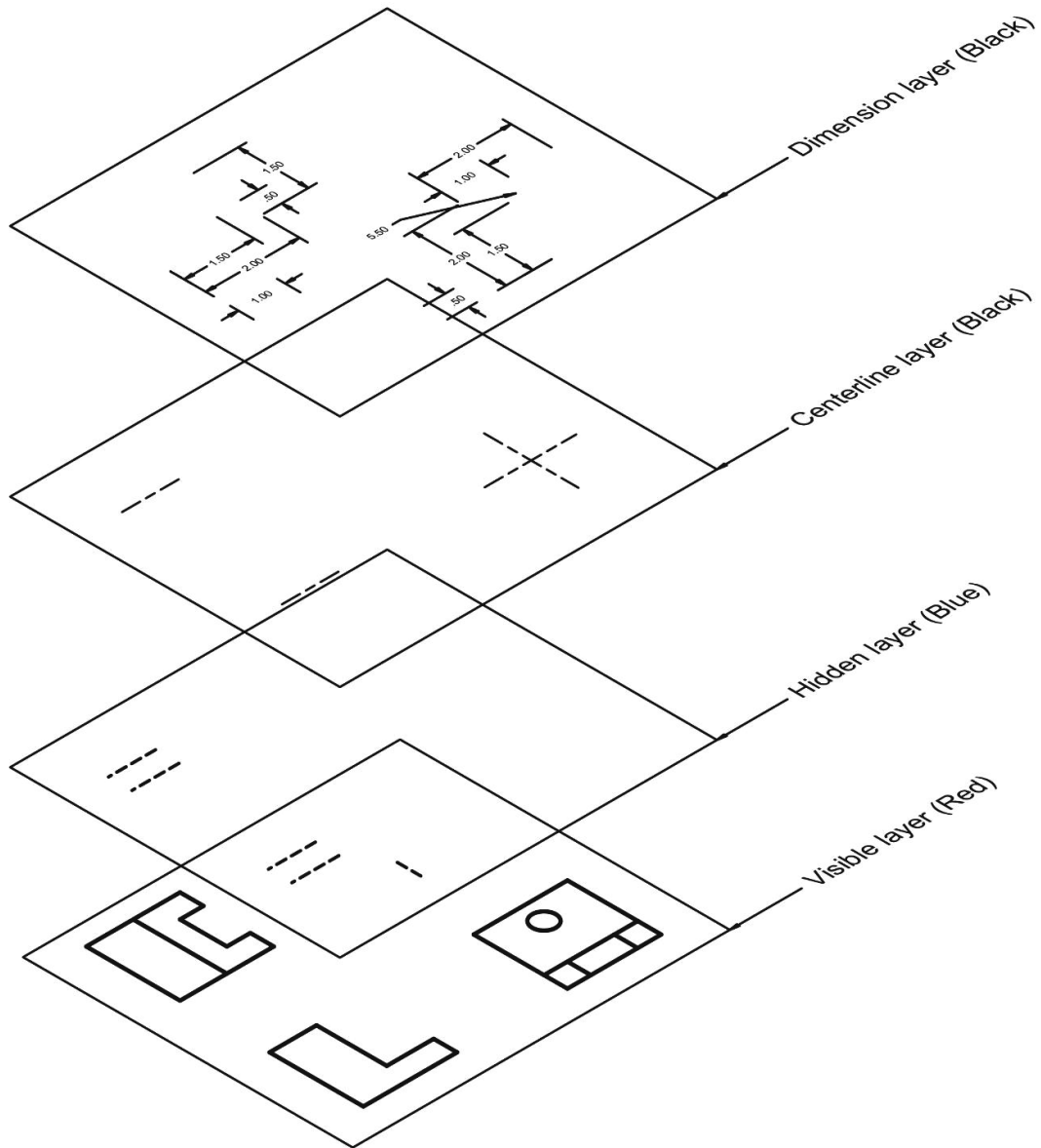
Figure 5.2-2: Layer organization of an orthographic projection
