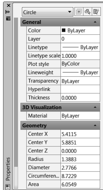
Figure 5.4-1: Properties window for a circle
