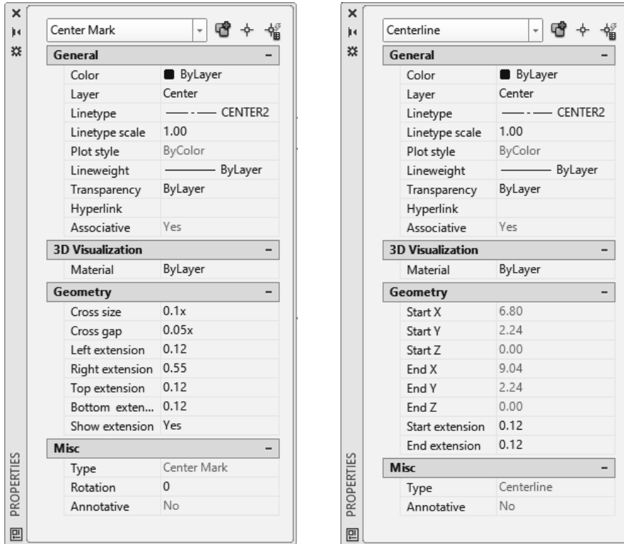
Figure 5.9-3: Center mark and center line Properties window
